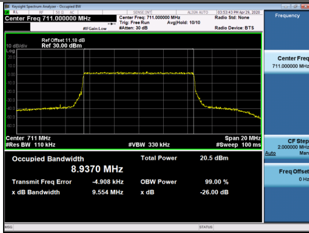
HCH_16QAM_50RB#0
