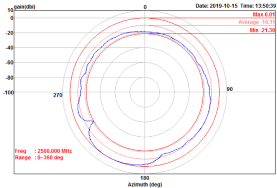
Figure 3. 2.4G Antenna 2500MHz
