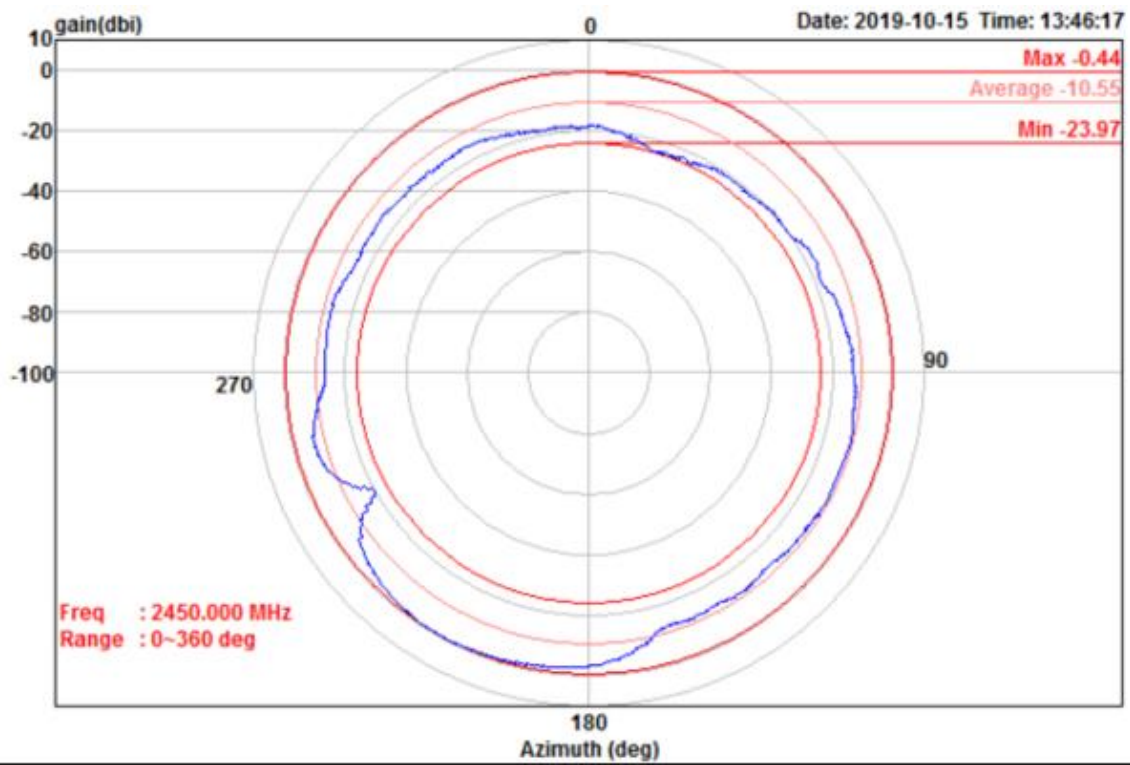
Figure 2. 2.4G Antenna 2450MHz
