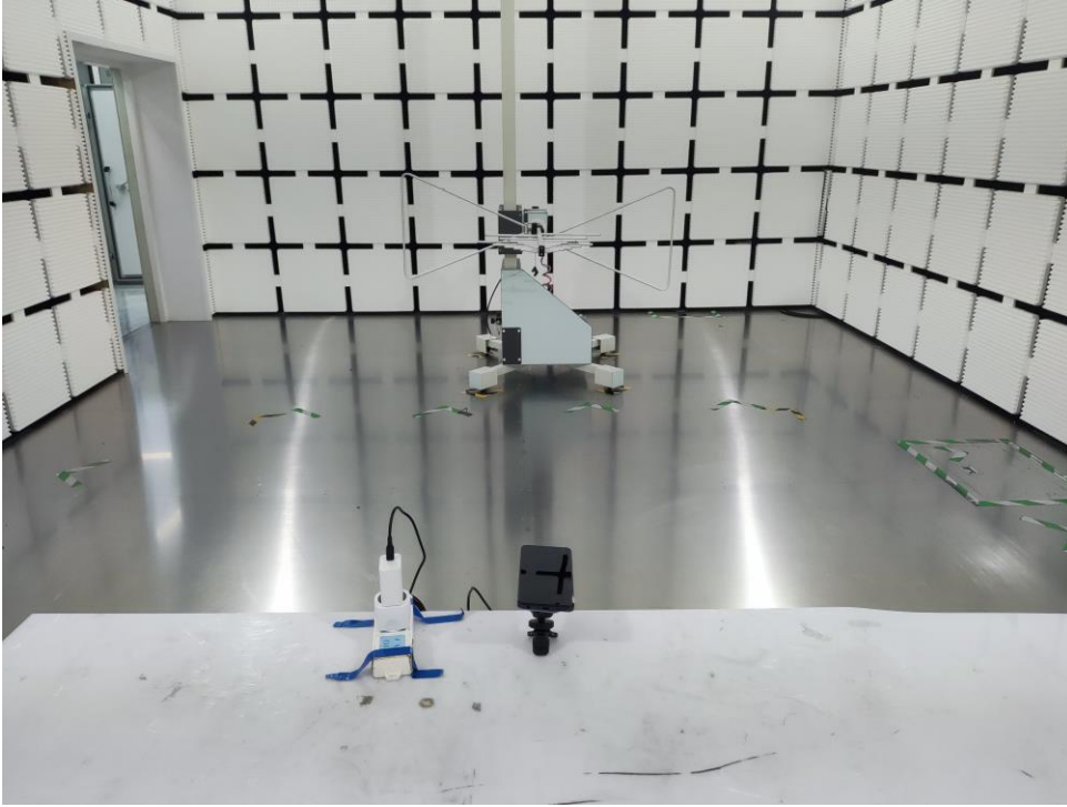
Radiation (30MHz-1000MHz)
