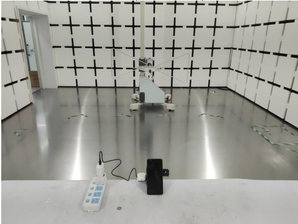
Radiation (30MHz-1000MHz)
