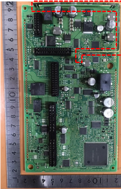
Component side
