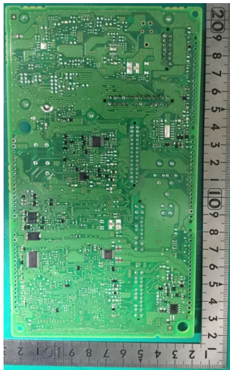
Solder side
