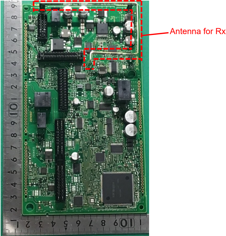
Component side
