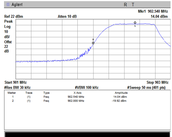
Plot 7.4.3 The highest band edge emission at low carrier frequency
