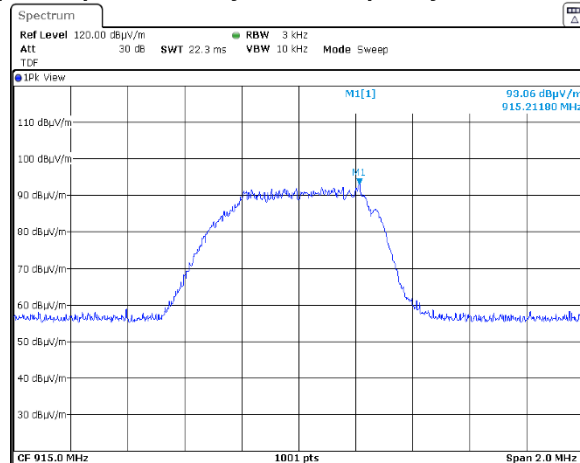
Plot 7.5.5 Peak spectral power density at mid frequency with bitrate 21.9 kbps
