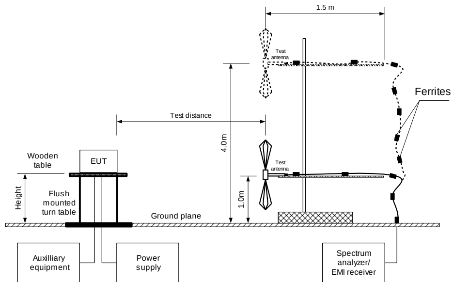
Figure 7.3.1 Setup for carrier field strength measurements
