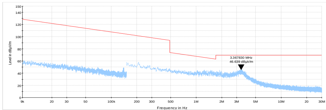
Plot 7.2.5 Radiated emission measurements from 9 kHz to 30 MHz at the mid carrier frequency
