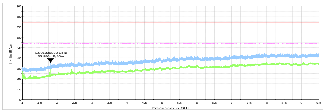
Plot 7.2.11 Radiated emission measurements from 1000 to 9500 MHz at the mid carrier frequency
