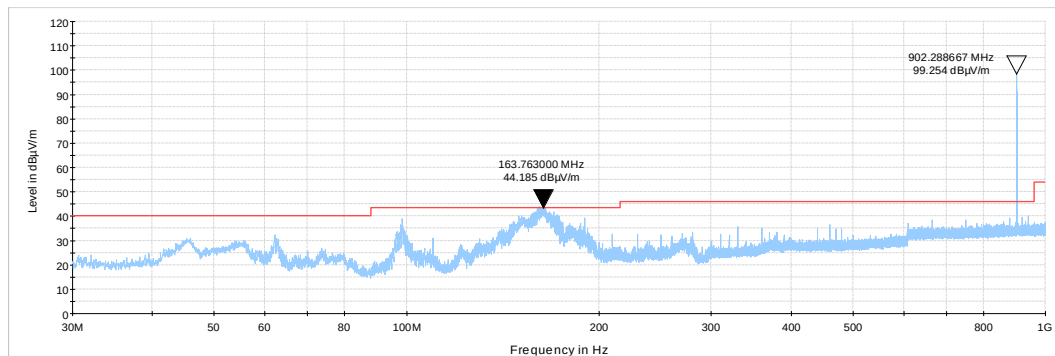
Plot 7.2.8 Radiated emission measurements from 30 to 1000 MHz at the mid carrier frequency
