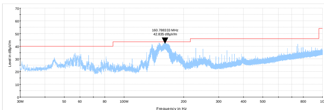
Plot 8.2.2 Radiated emission measurements in 30 – 1000 MHz range, vertical and horizontal antenna polarization
