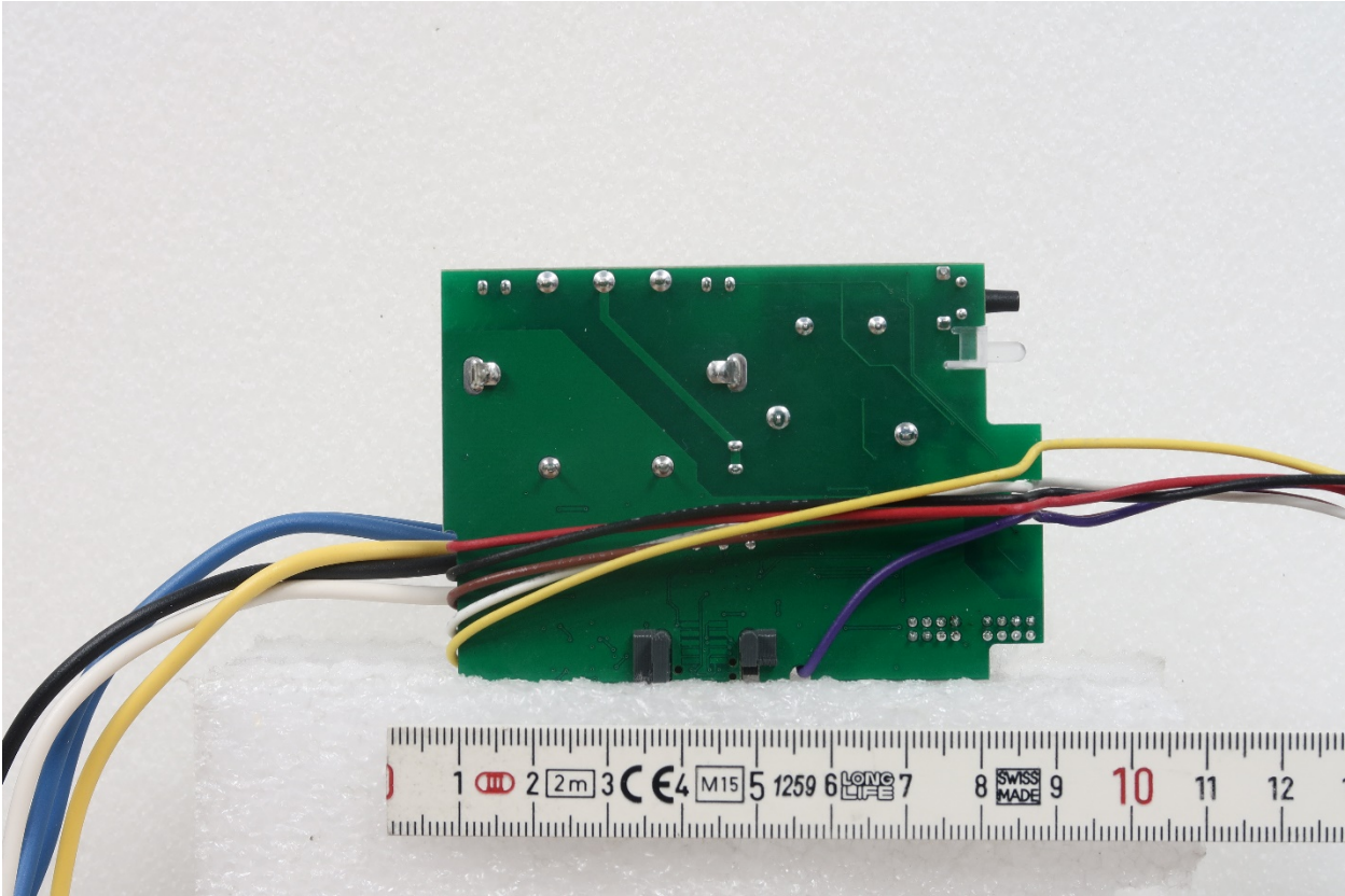
Mainboard Rear
