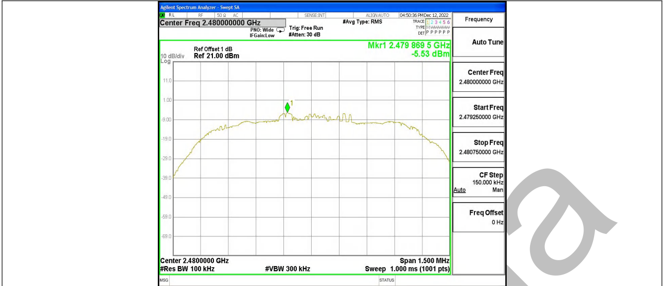
3DH5_Ant1_2480_0~Reference
