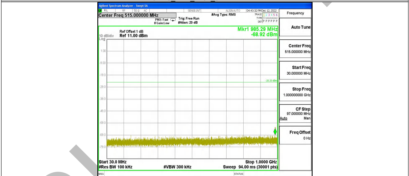
3DH5_Ant1_2402_30~1000
