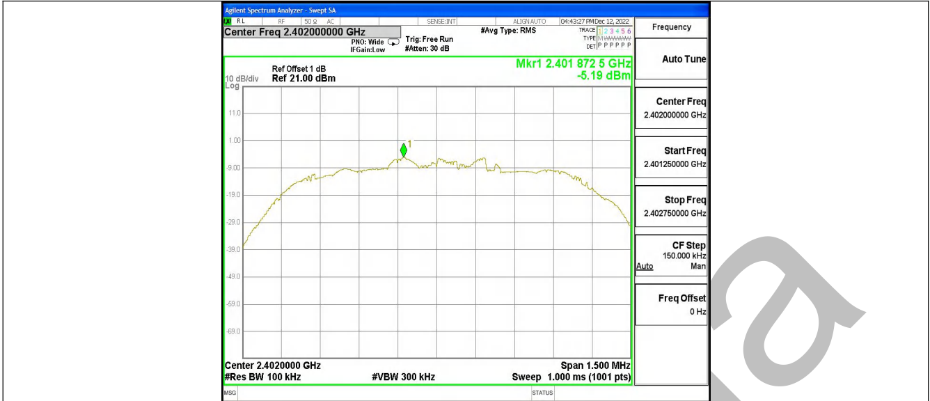
3DH5_Ant1_2402_0~Reference
