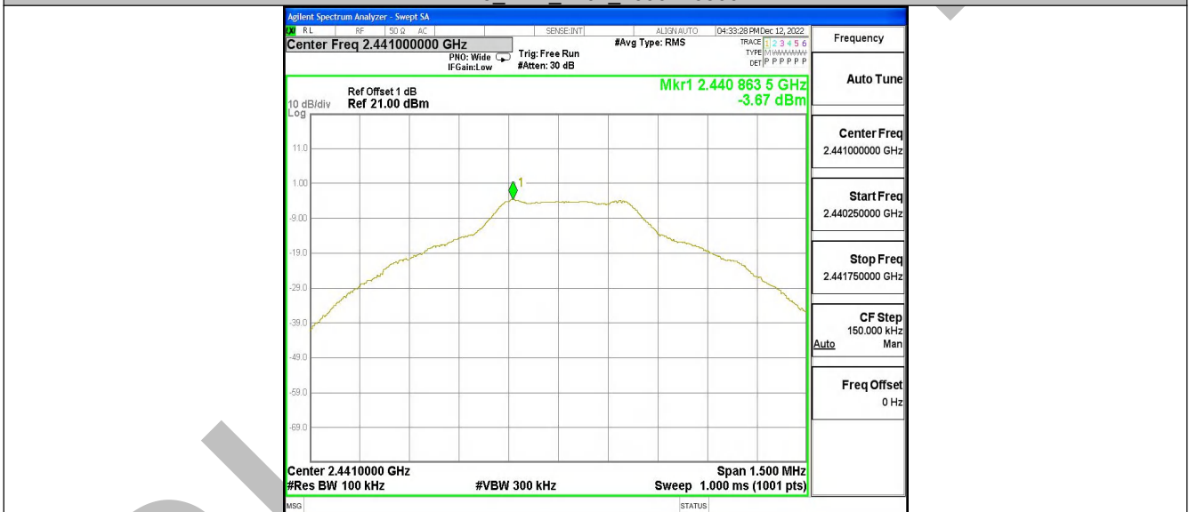
DH5_Ant1_2441_0~Reference
