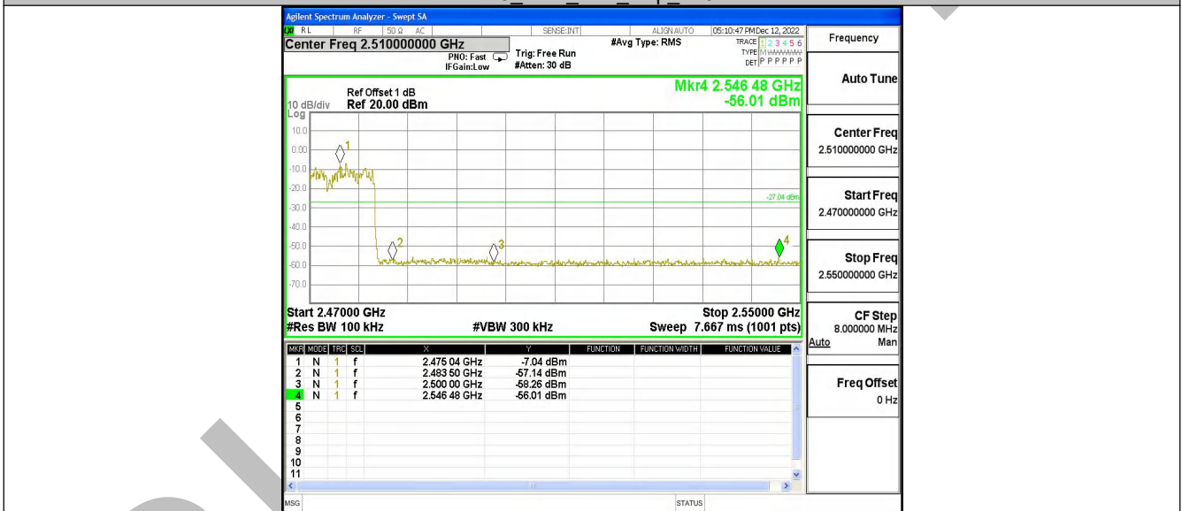
2DH5_Ant1_High_Hop_2480
