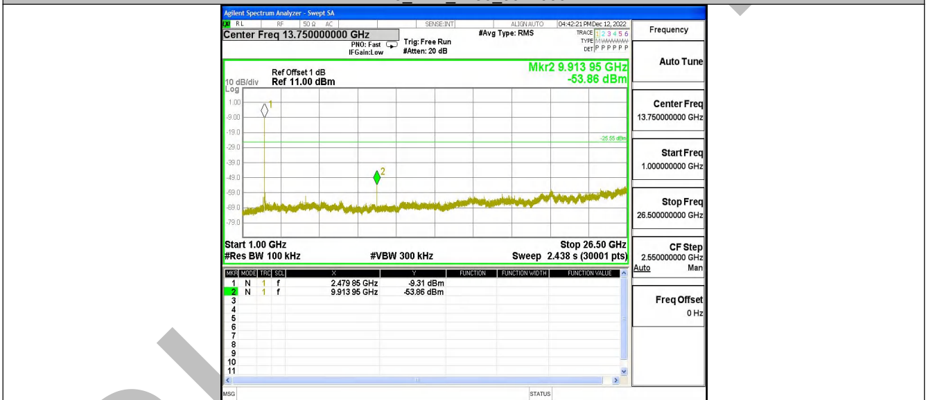
2DH5_Ant1_2480_1000~26500
