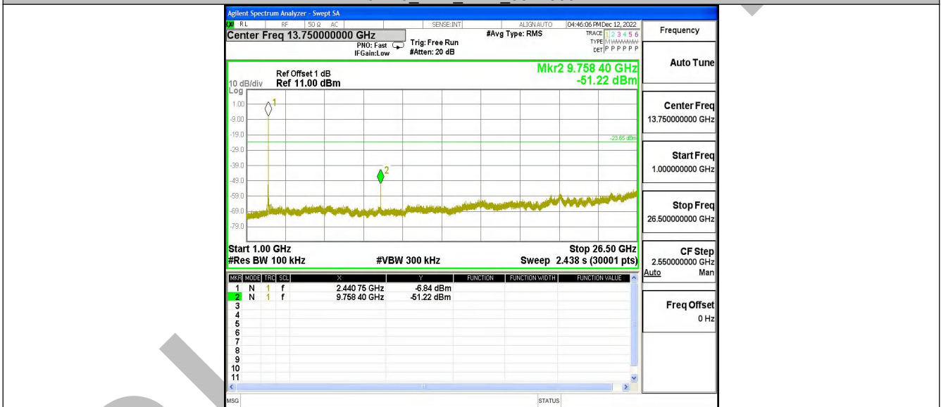
3DH5_Ant1_2441_1000~26500
