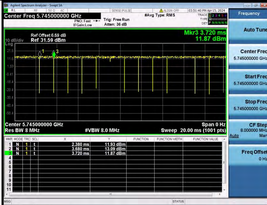
Duty Cycle NVNT_ANT1_802_11n(HT20)_5745
