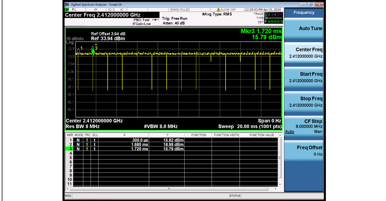
Duty Cycle_NVNT_ANT1_802_11g_2412
