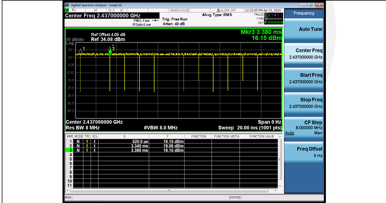
Duty Cycle_NVNT_ANT1_802_11g_2437
