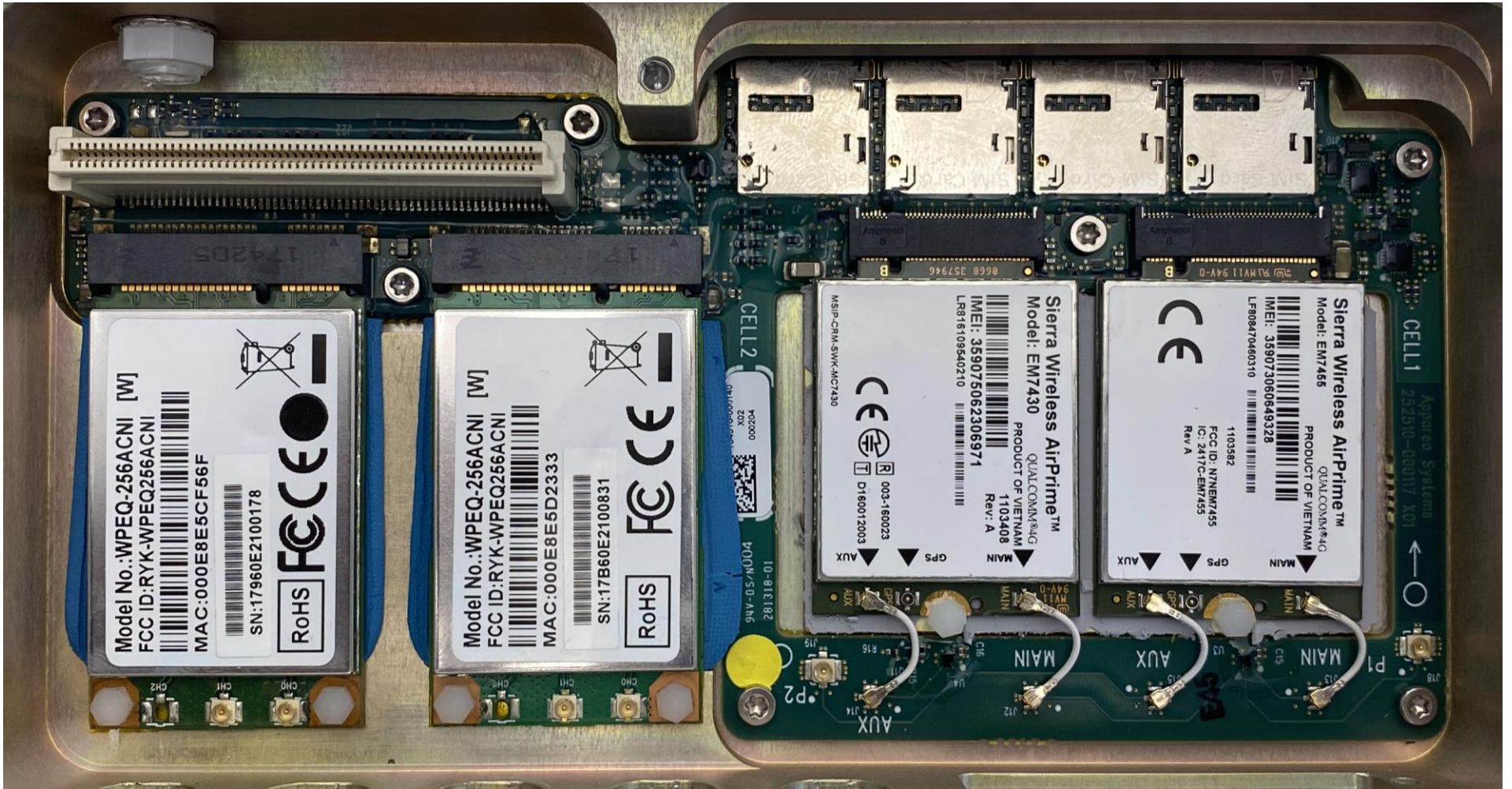
AFS6460 – Unit Internal with Modules
