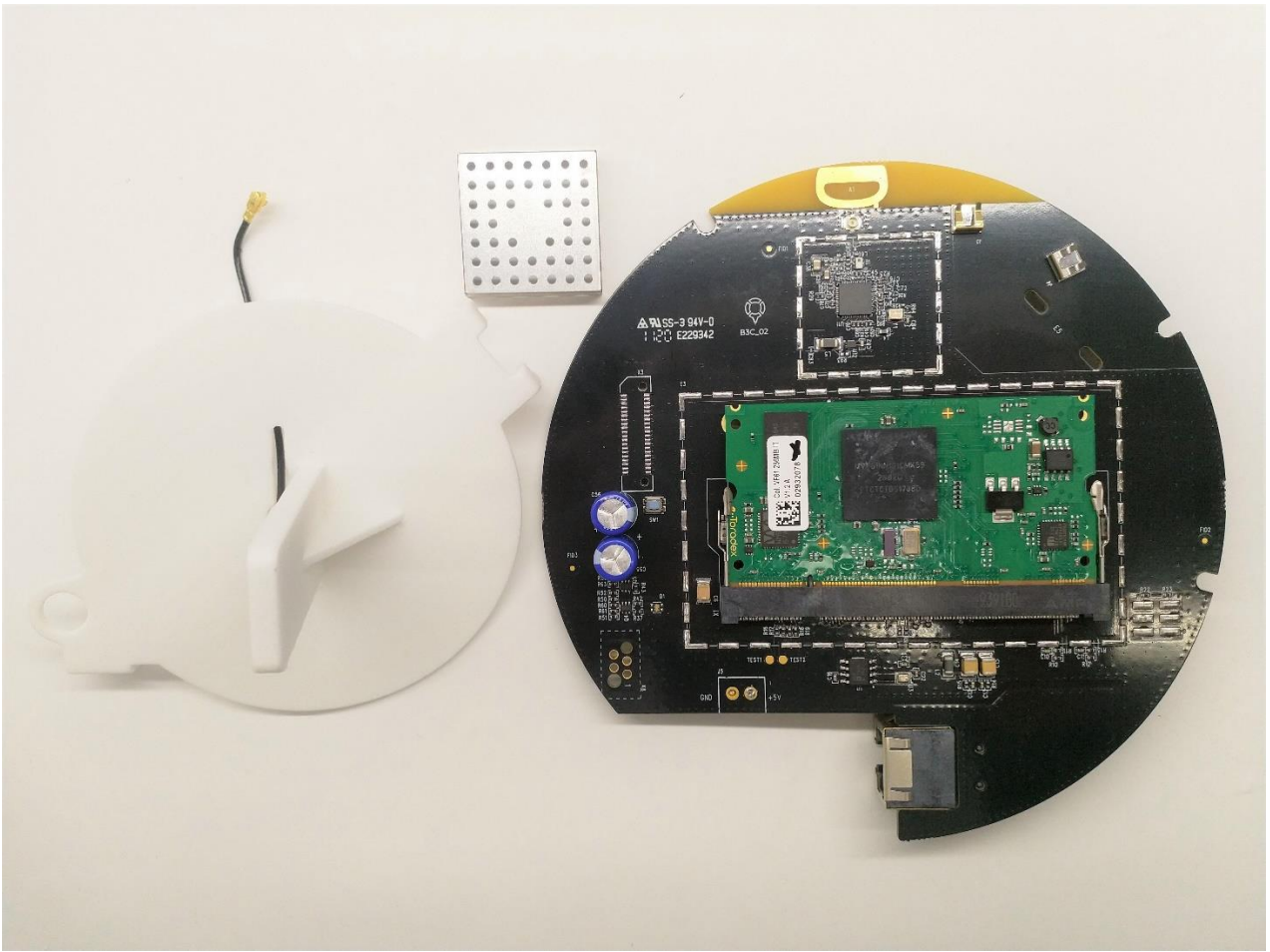
Beacon PCB top side
