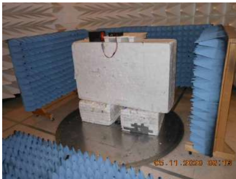
Test Setup
