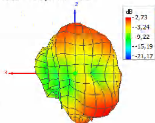
Theta = 90, Phi = 90
