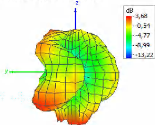
Theta = 90, Phi = 180
