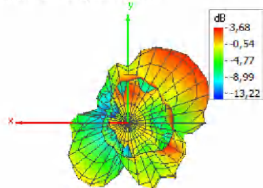
Theta = 180, Phi = 0
