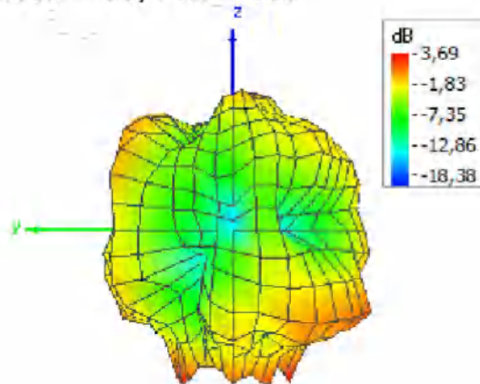
Theta = 90, Phi = 180
