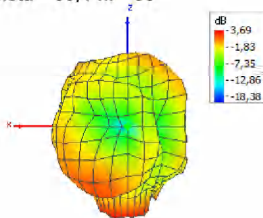
Theta = 90, Phi = 90
