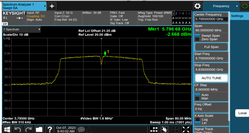
11N40MIMO Ant2 5795
