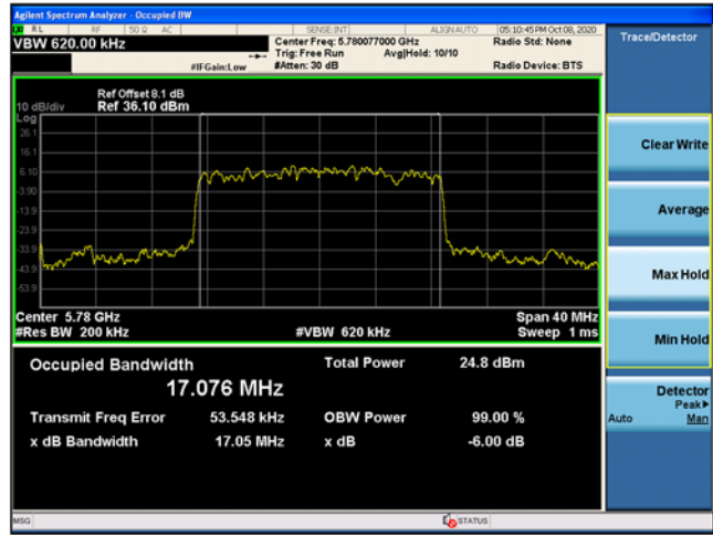
Middle Channel 5780.077 MHz
