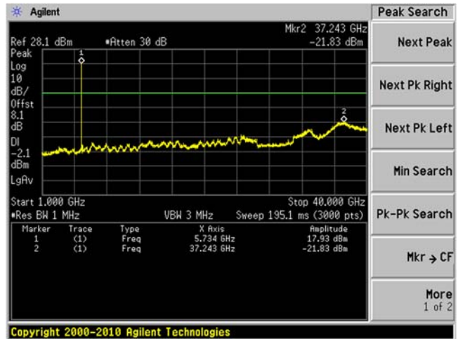
Middle Channel 1 GHz – 40 GHz
