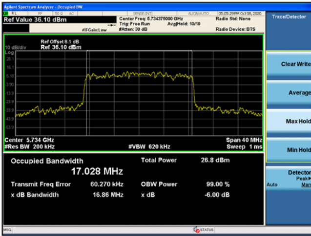
Low Channel 5734.375 MHz
