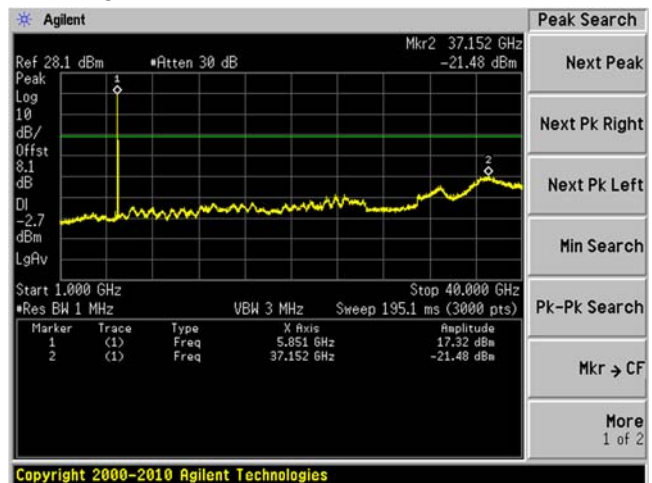
High Channel 1 GHz – 40 GHz
