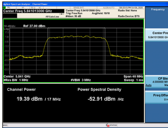
High Channel 5841.013 MHz
