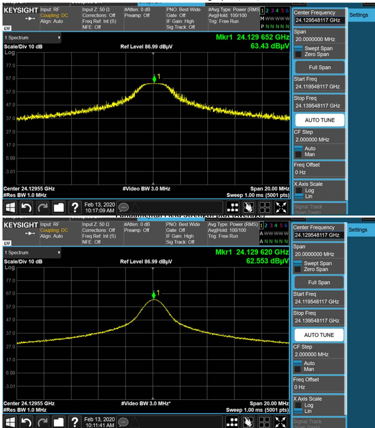
Fundamental Field Strength plot (Peak)
