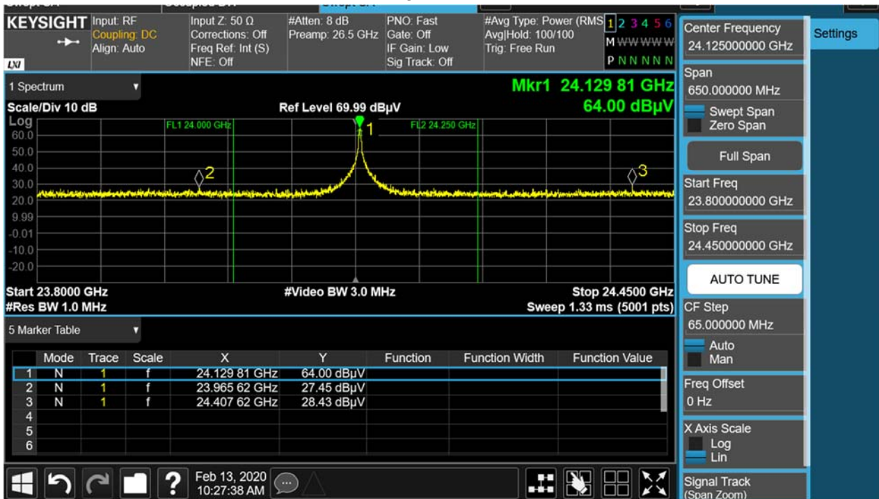
Band Edge Plot(peak, x-V)
