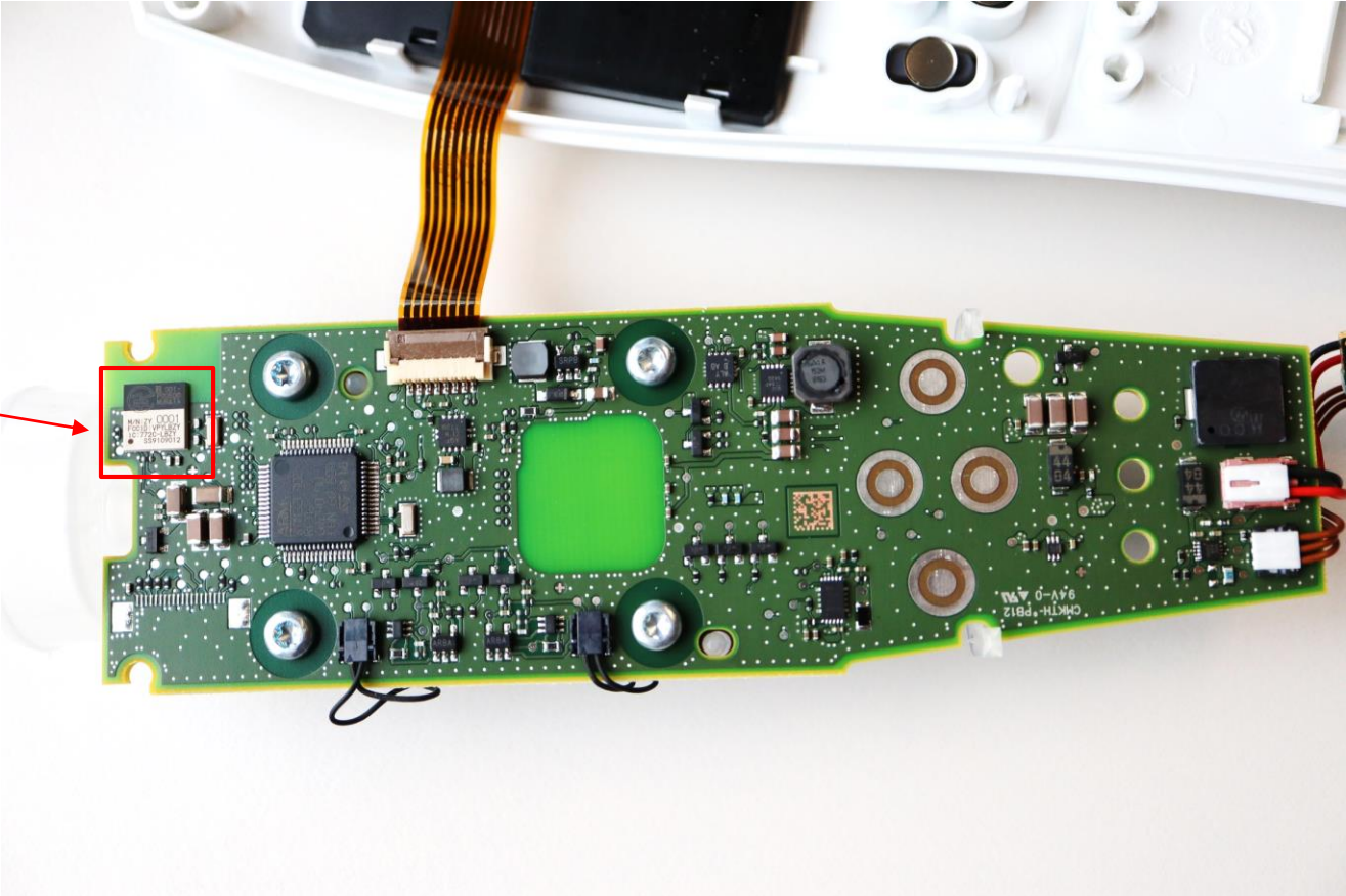
BLE Module with integrated antenna
