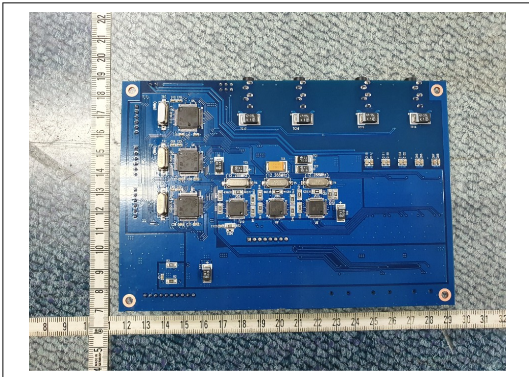
MainBoard-Rear
