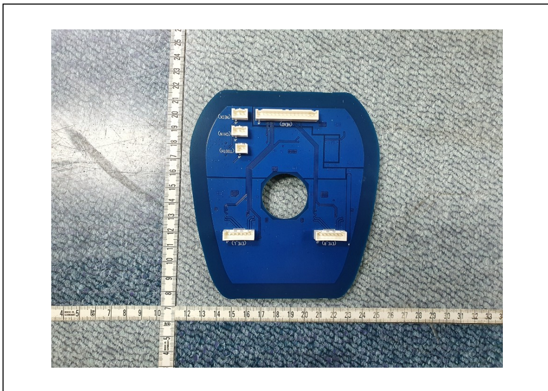
SubBoard-Rear
