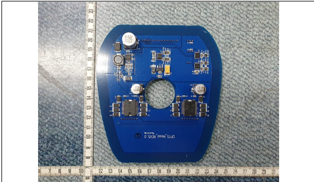
SubBoard-Front
