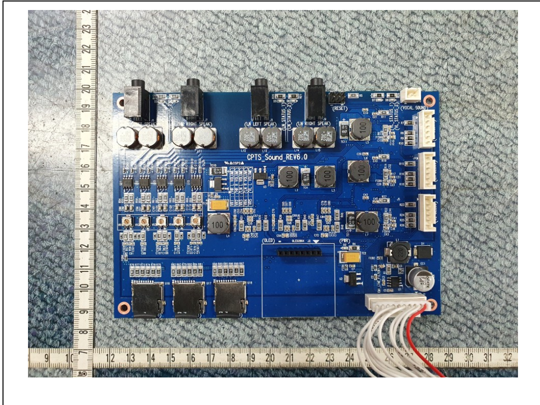
MainBoard-Rear
