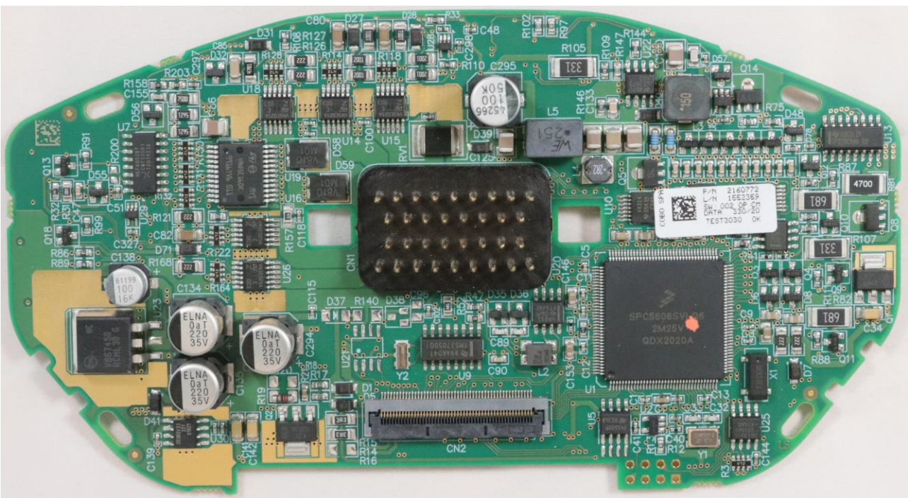
Bottom View
