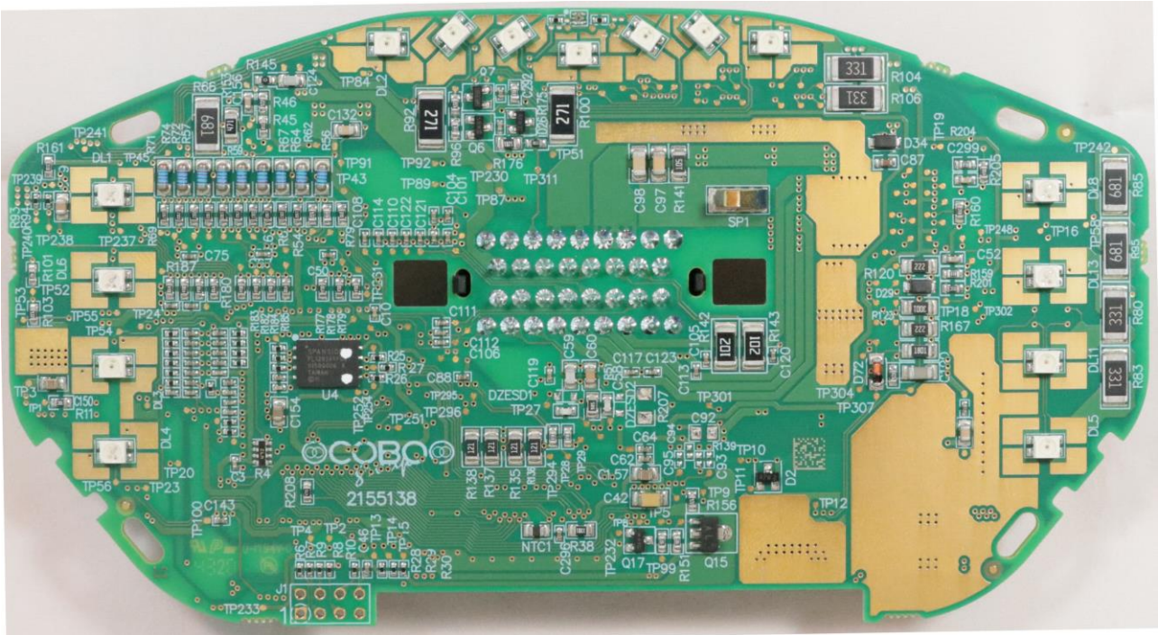
Top View
