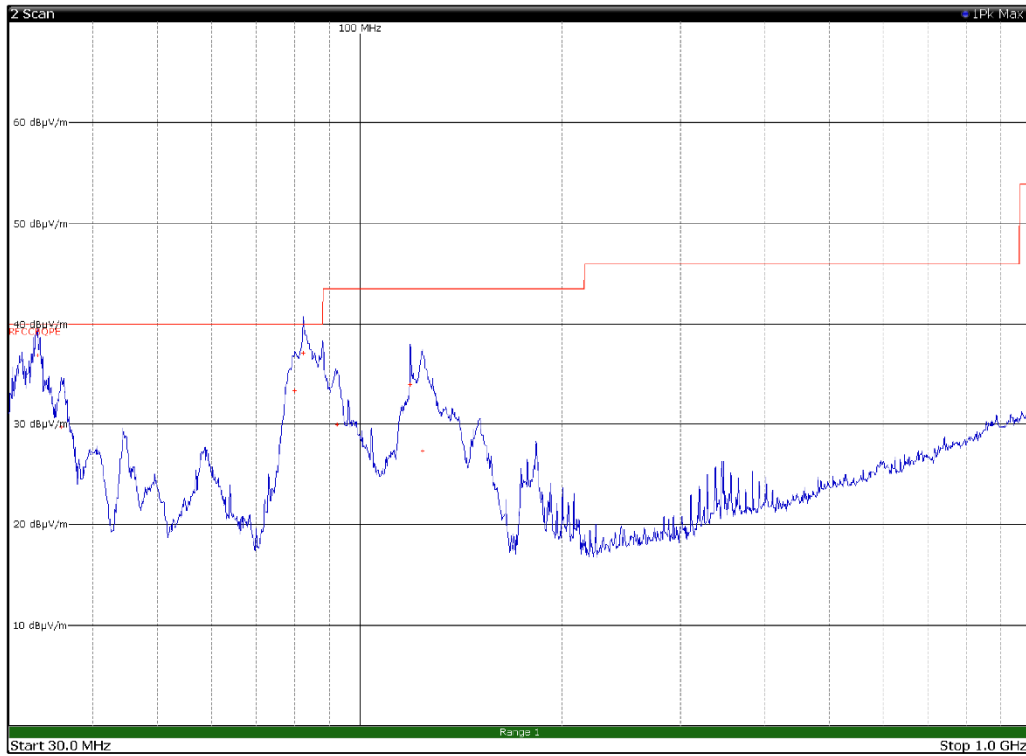
Vertical polarization
