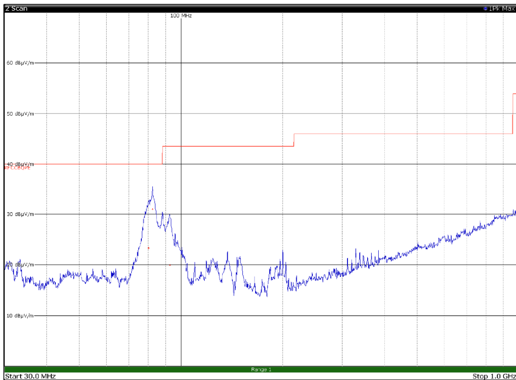
Horizontal polarization
