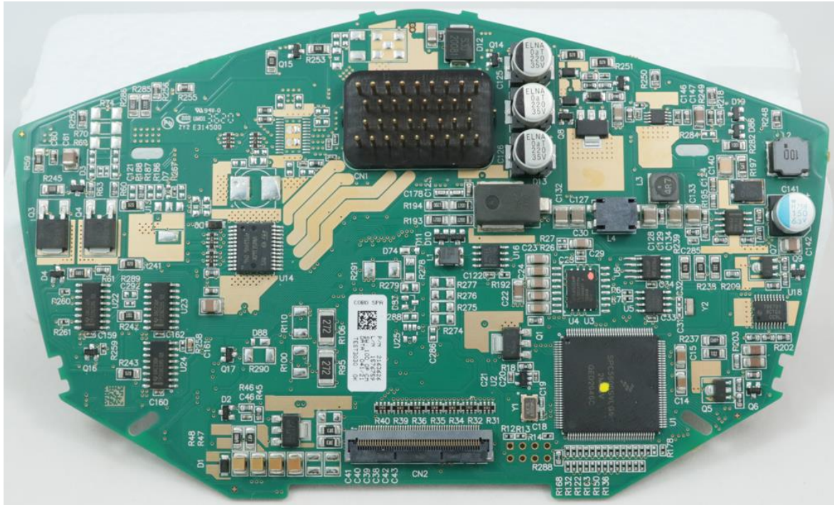
Bottom view
