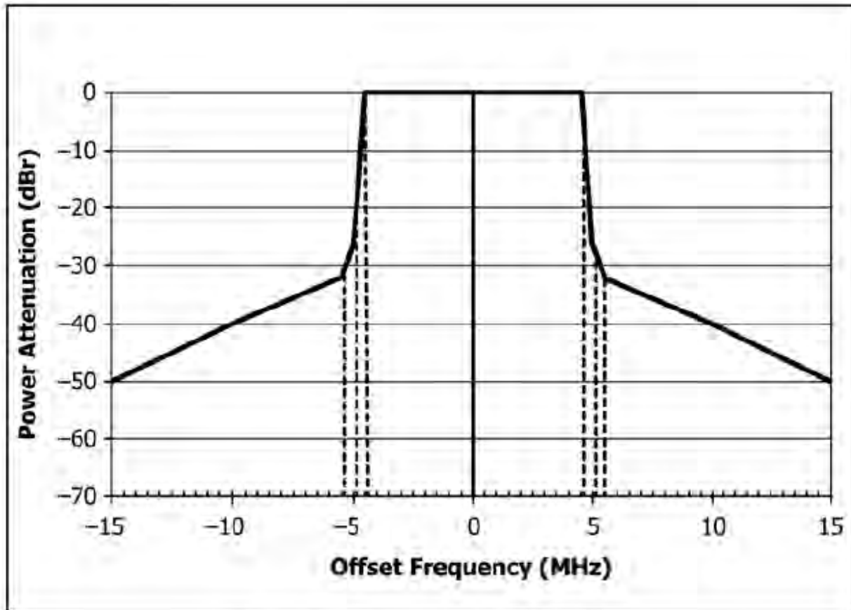
FIG. 14 Class C Transmitter Spectrum Mask
