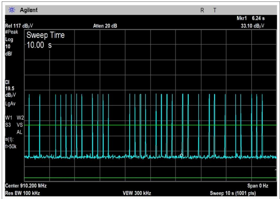
10 second observation window
