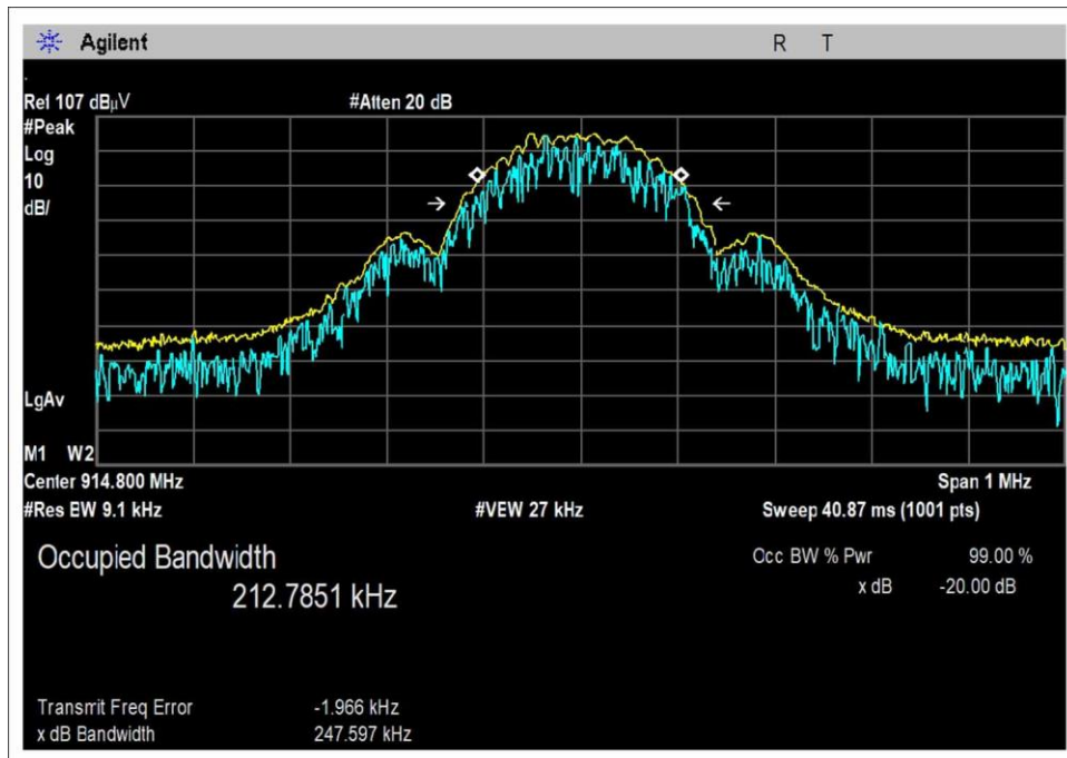
Antenna 1; Middle Channel
