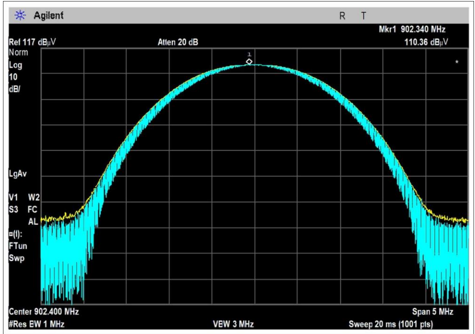
Antenna 0; Low Channel
