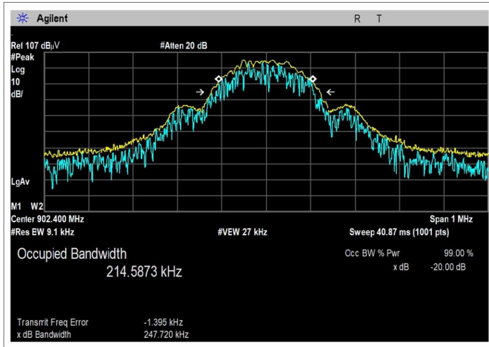
Antenna 1; Low Channel
