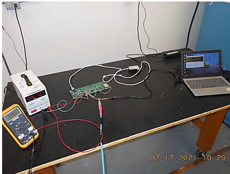
Voltage Variation
