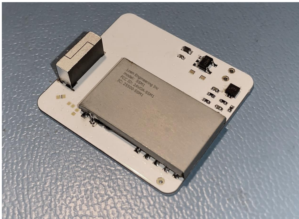
Top View with Antenna, Mounted on Host Board
