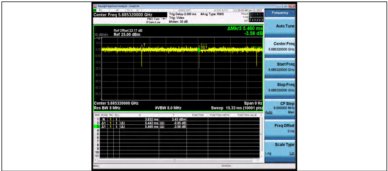
11AX80_RU_Ant2_5690_996Tone_RU67
