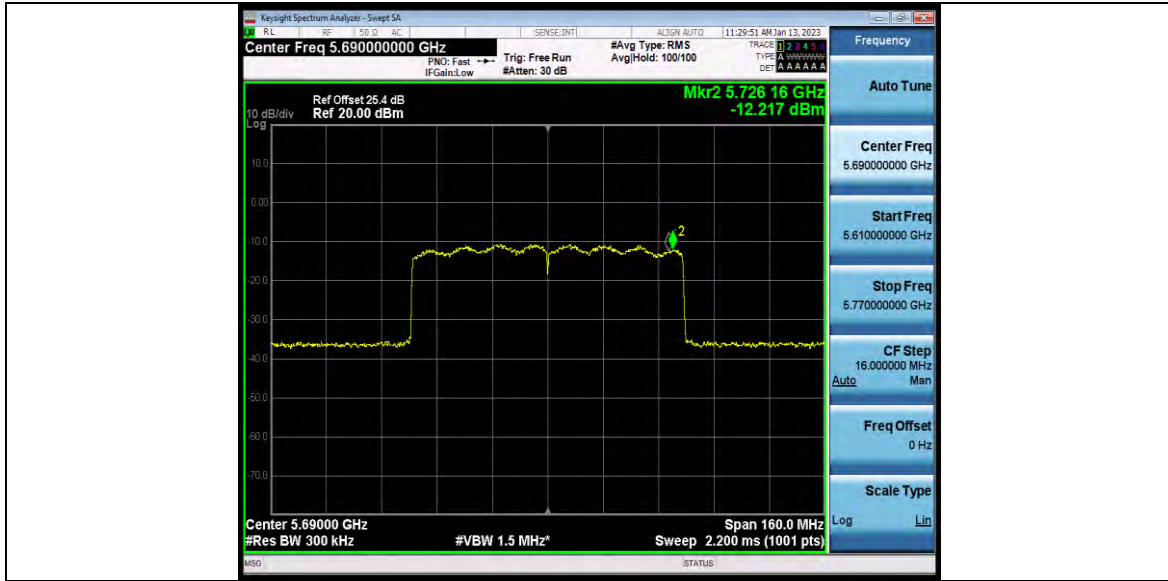
11AX80_RU_Ant2_5690_UNII-3_996Tone_RU67
