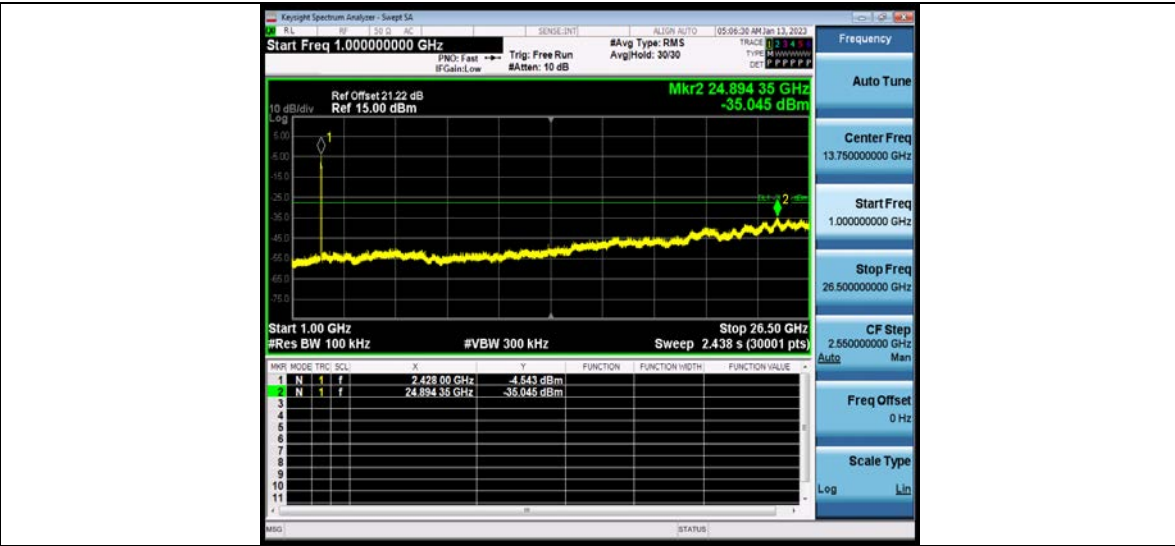
11AX40_RU_Ant2_2437_484Tone_RU65_0-Reference
