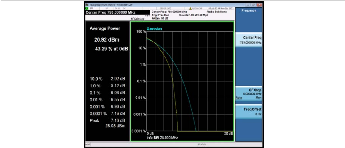
Band14-5MHz-16QAM-23355-1RB#0
