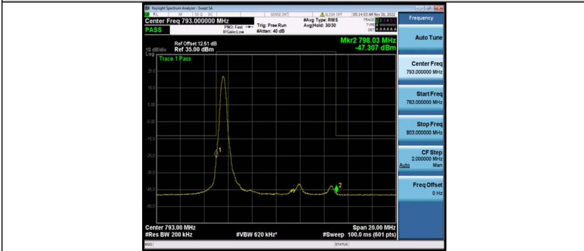
Band14-10MHz-QPSK-23330-1RB#49
