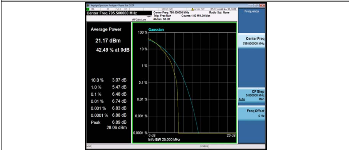
Band14-5MHz-64QAM-23355-25RB#0
