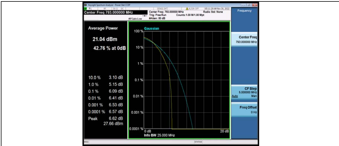
Band14-5MHz-64QAM-23330-25RB#0
