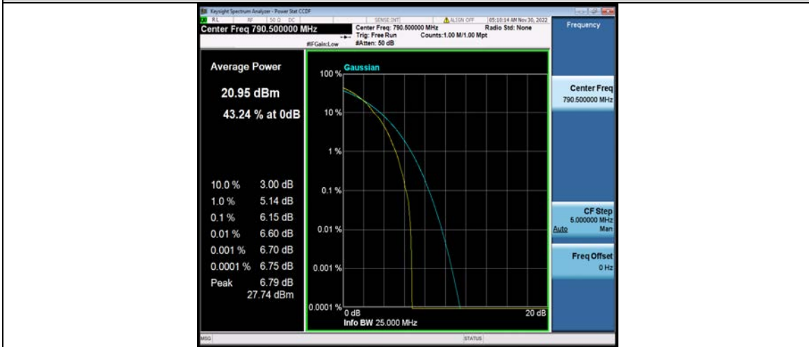
Band14-5MHz-64QAM-23305-25RB#0
