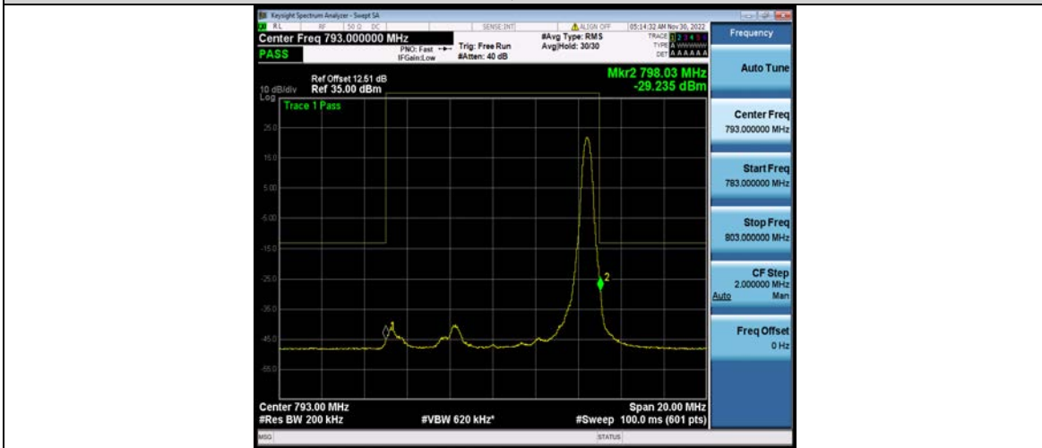
Band14-10MHz-QPSK-23330-50RB#0
