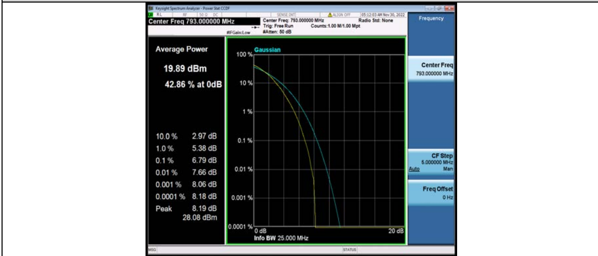
Band14-5MHz-64QAM-23355-1RB#0
