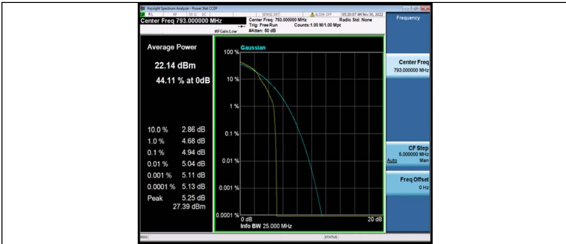
Band14-10MHz-16QAM-23330-50RB#0
