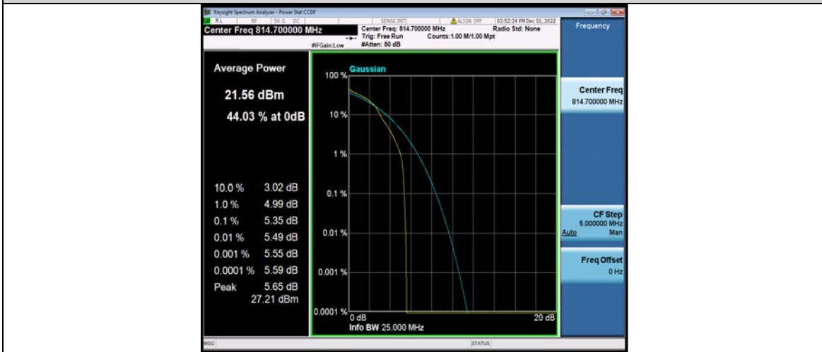
Band26-1.4MHz-16QAM-26697-6RB#0
