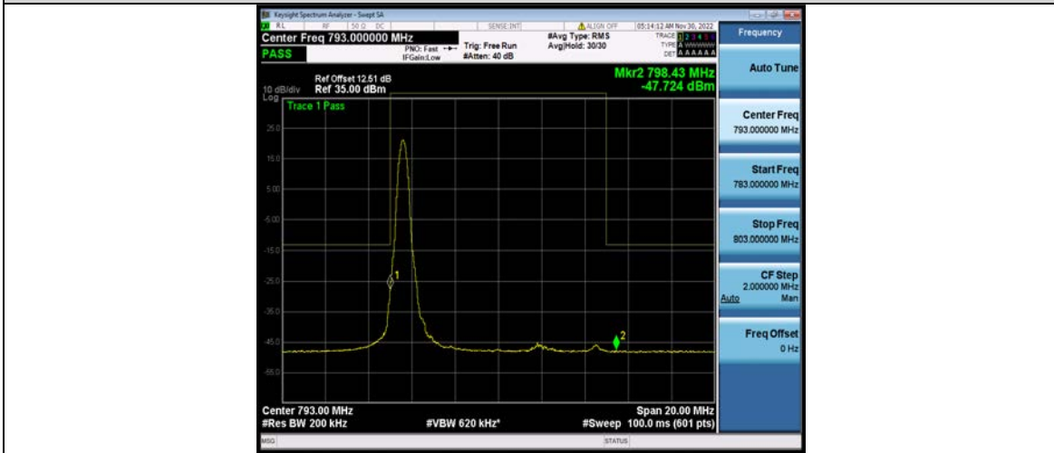
Band14-10MHz-16QAM-23330-1RB#49
