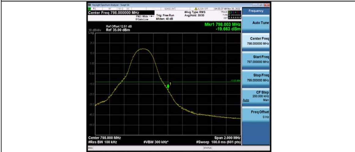
Band14-5MHz-16QAM-23355-25RB#0
