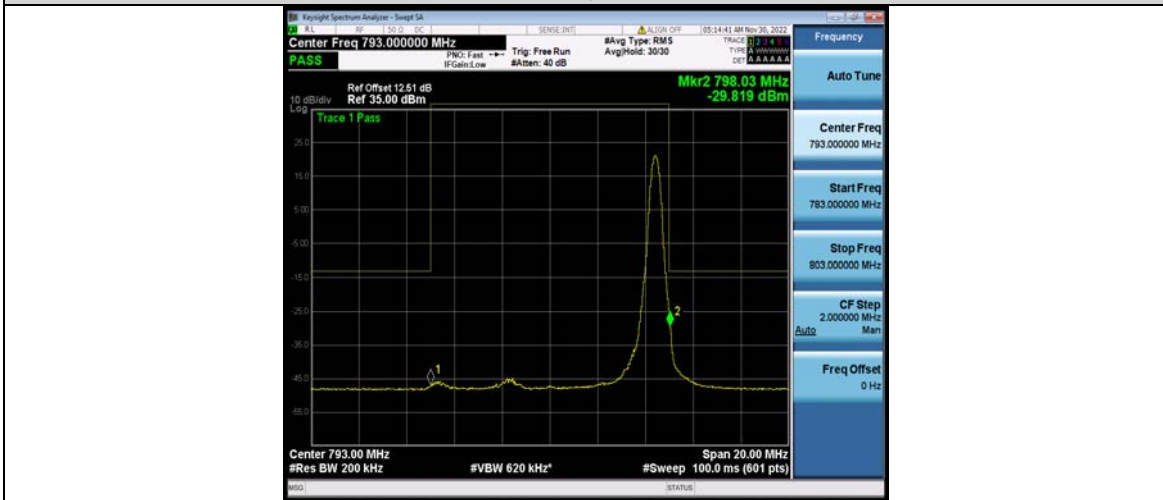
Band14-10MHz-16QAM-23330-50RB#0
