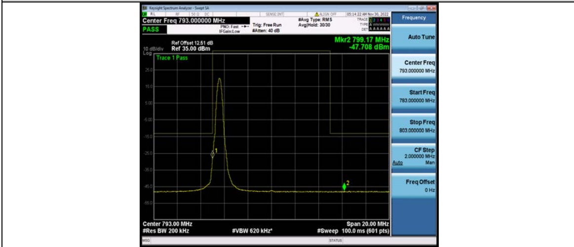
Band14-10MHz-64QAM-23330-1RB#49
