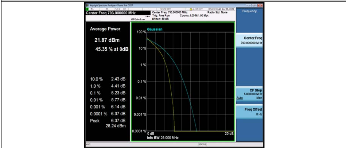
Band14-10MHz-16QAM-23330-1RB#0
