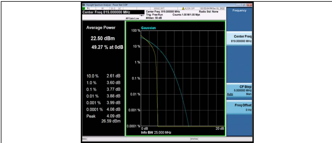
Band26-1.4MHz-QPSK-26740-6RB#0
