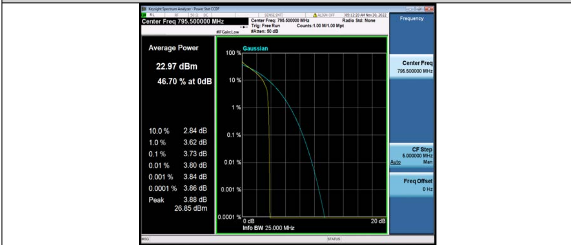
Band14-5MHz-QPSK-23355-25RB#0
