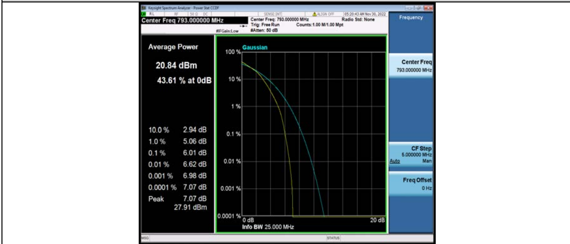
Band14-10MHz-64QAM-23330-1RB#0
