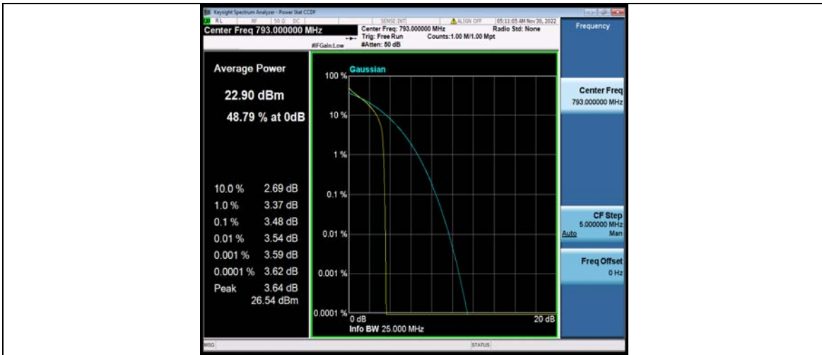
Band14-5MHz-QPSK-23330-25RB#0
