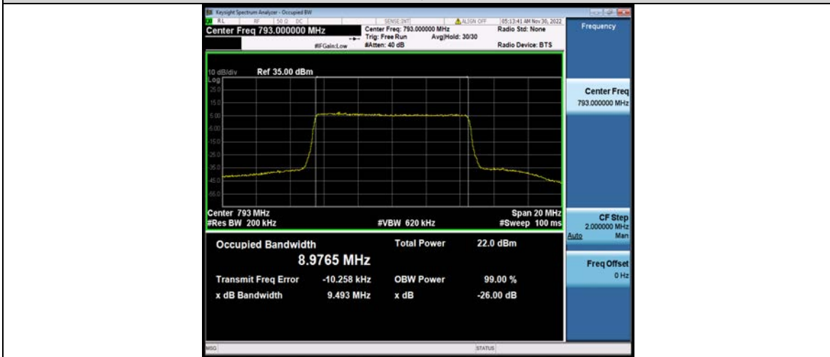
Band14-10MHz-64QAM-23330-50RB#0
