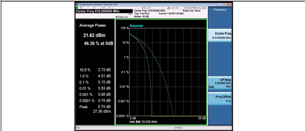
Band26-1.4MHz-QPSK-26783-1RB#0
