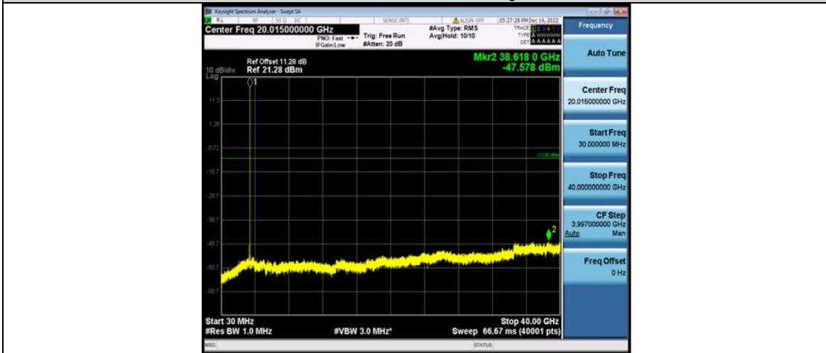
Band42-20MHz-QPSK-42590-1RB#0-Range1:30~40000MHz
