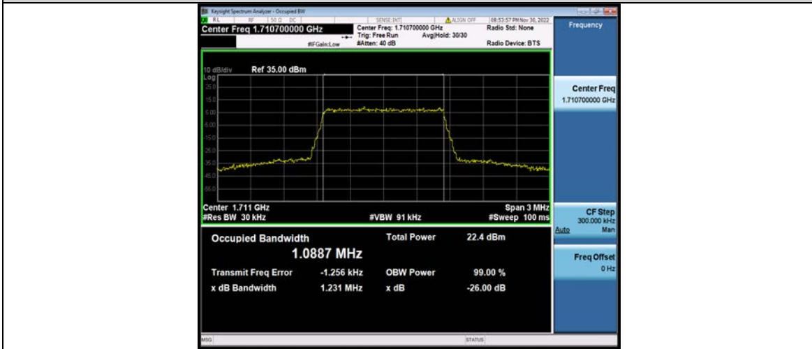
Band66-1.4MHz-64QAM-132322-6RB#0
