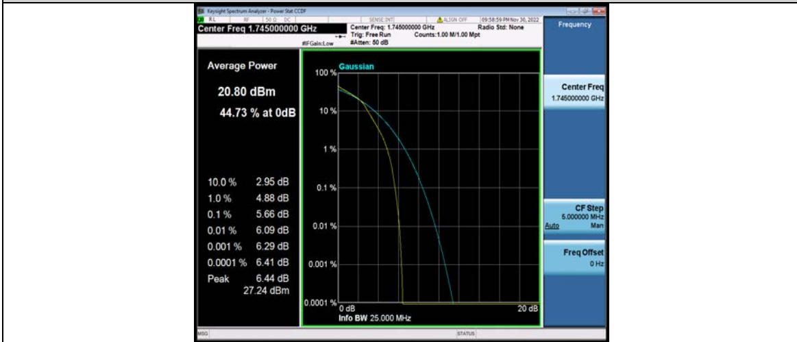
Band66-5MHz-16QAM-132647-1RB#0
