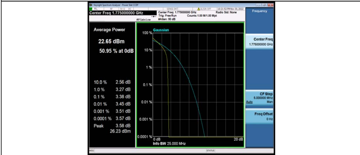
Band66-10MHz-QPSK-132622-50RB#0
