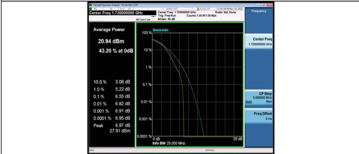
Band66-20MHz-64QAM-132072-100RB#0
