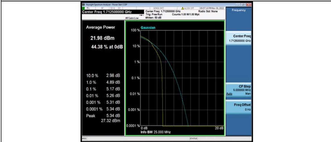
Band66-5MHz-16QAM-131997-25RB#0
