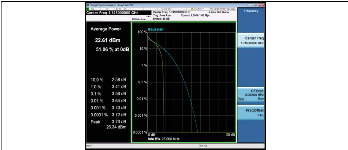
Band66-1.4MHz-QPSK-132322-6RB#0
