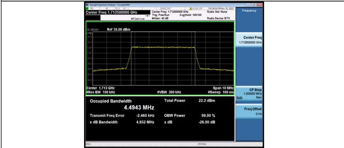
Band66-5MHz-64QAM-132322-25RB#0
