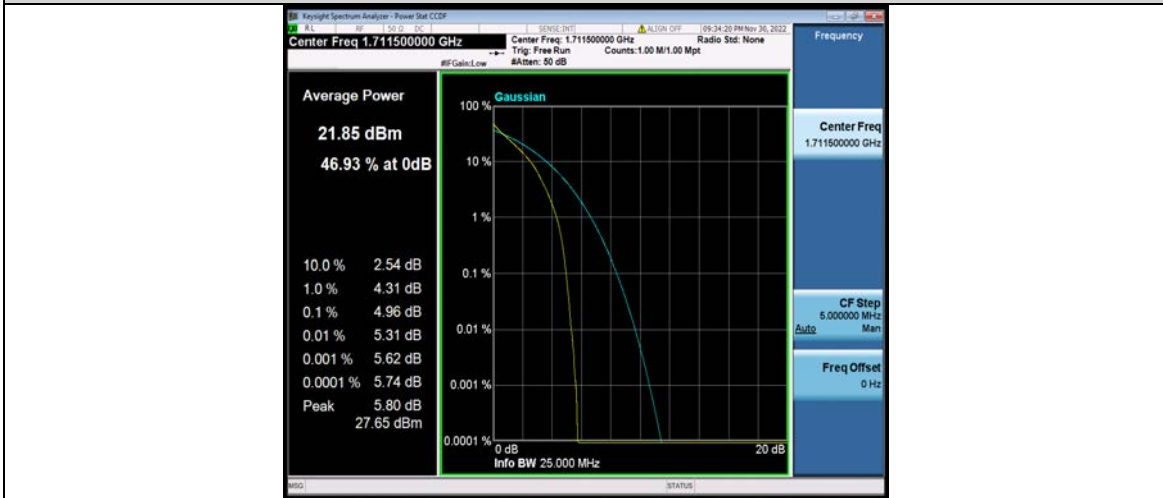
Band66-3MHz-QPSK-132322-1RB#0
