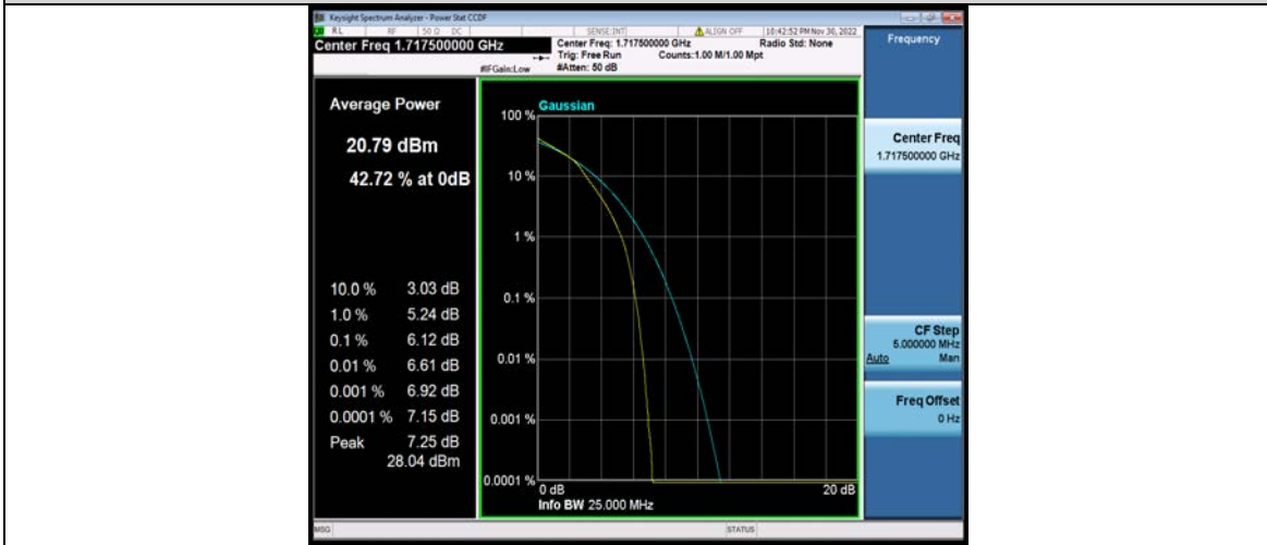
Band66-15MHz-16QAM-132322-1RB#0
