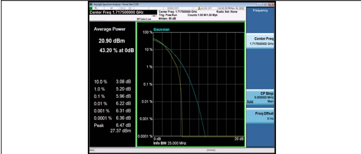
Band66-15MHz-64QAM-132047-75RB#0
