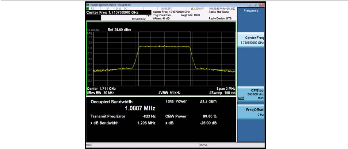
Band66-1.4MHz-16QAM-132322-6RB#0
