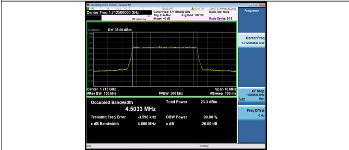
Band66-5MHz-16QAM-132322-25RB#0
