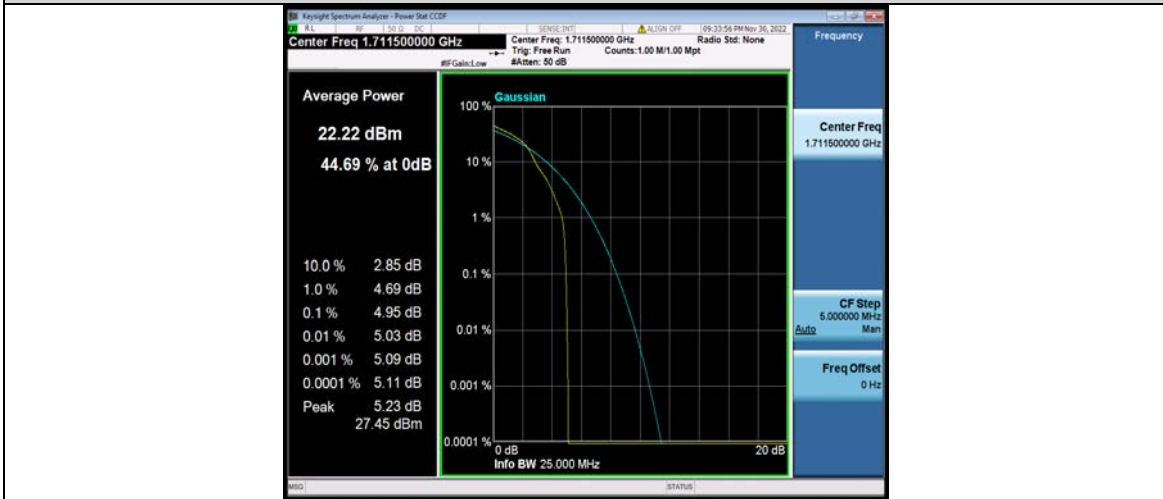
Band66-3MHz-16QAM-131987-15RB#0
