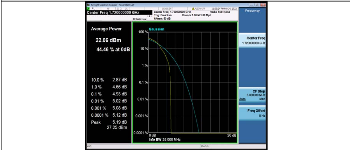
Band66-20MHz-16QAM-132072-100RB#0
