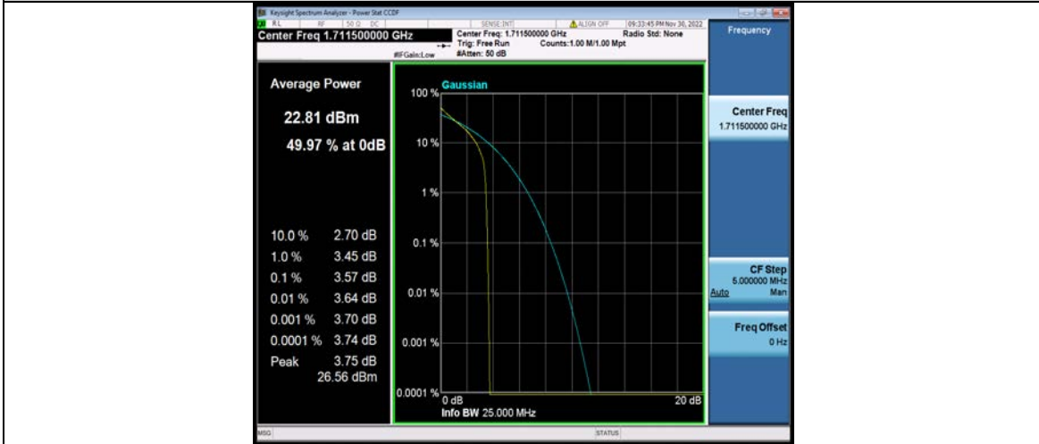
Band66-3MHz-QPSK-131987-15RB#0
