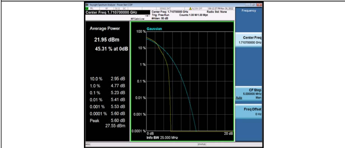
Band66-1.4MHz-16QAM-131979-6RB#0
