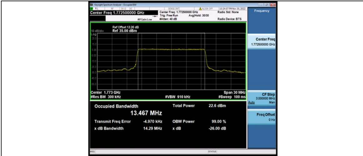
Band66-15MHz-16QAM-132047-75RB#0
