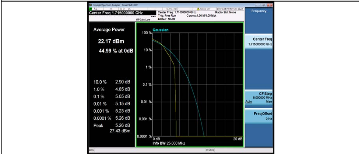
Band66-10MHz-16QAM-132022-50RB#0
