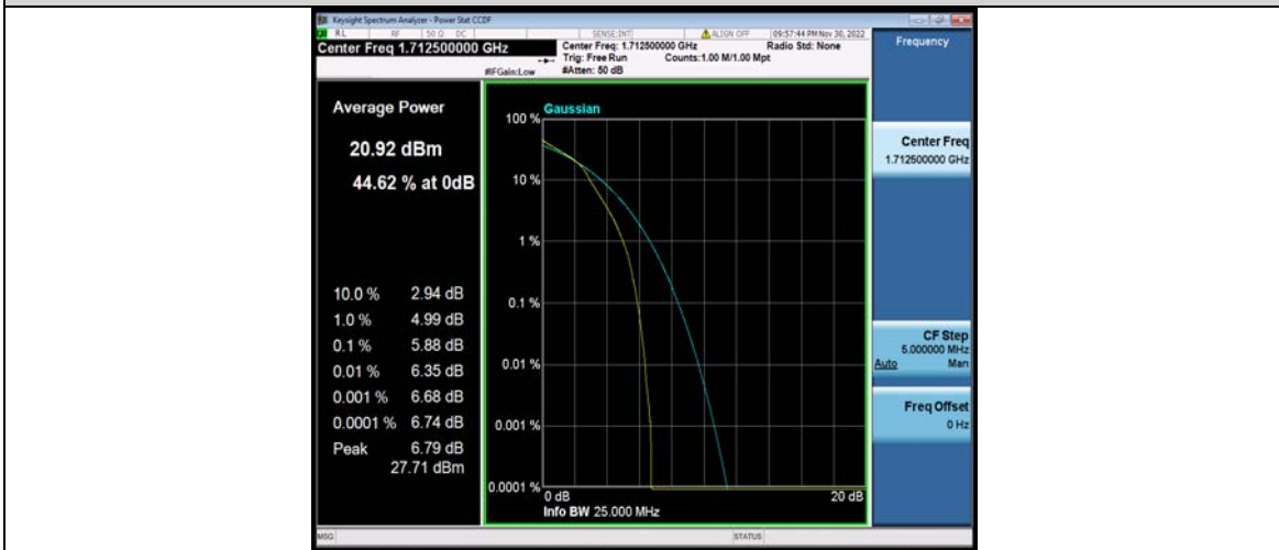
Band66-5MHz-16QAM-132322-1RB#0
