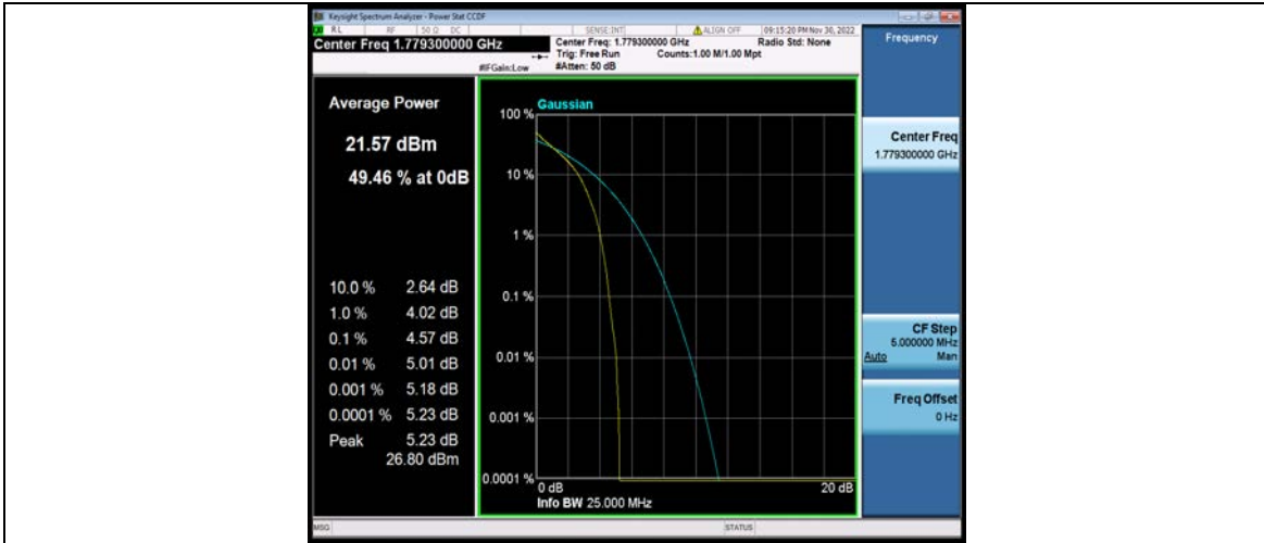
Band66-1.4MHz-16QAM-131979-1RB#0
