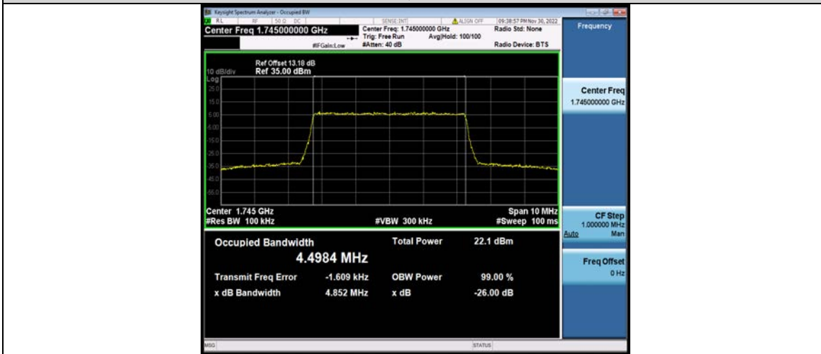
Band66-5MHz-64QAM-132647-25RB#0
