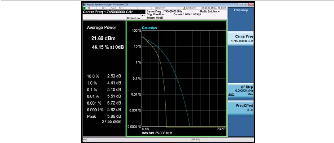
Band66-15MHz-QPSK-132597-1RB#0
