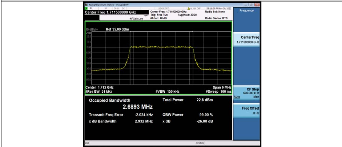
Band66-3MHz-16QAM-132322-15RB#0
