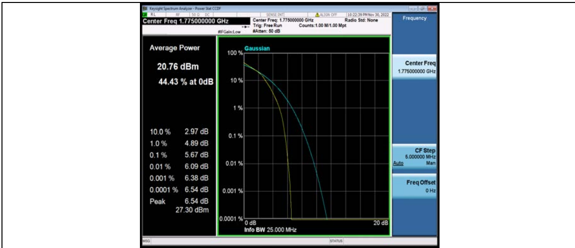
Band66-10MHz-64QAM-132022-1RB#0
