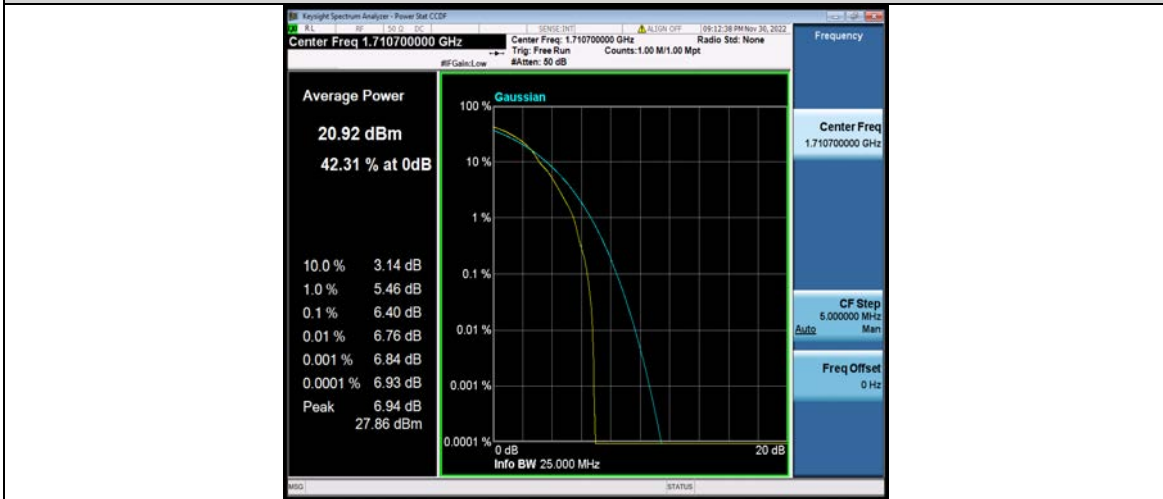
Band66-1.4MHz-64QAM-131979-6RB#0
