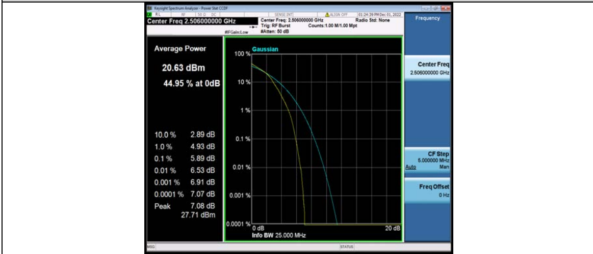
Band41-20MHz-16QAM-40620-1RB#0
