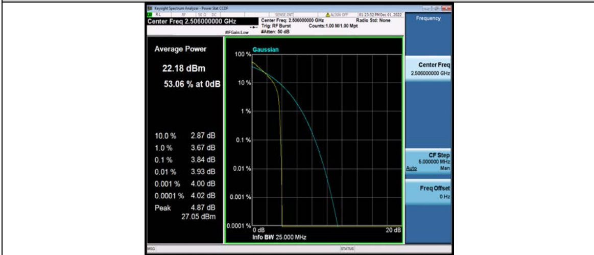
Band41-20MHz-QPSK-39750-100RB#0
