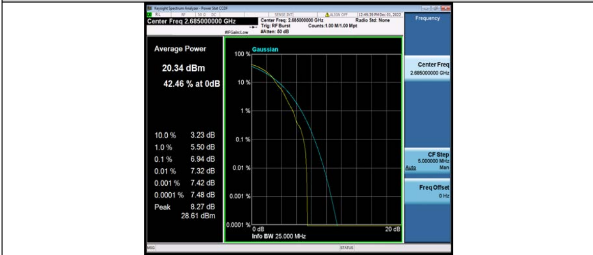
Band41-10MHz-64QAM-41540-50RB#0
