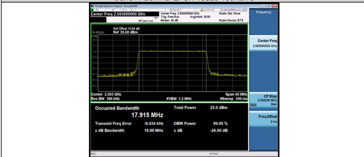
Band41-20MHz-QPSK-41490-100RB#0
