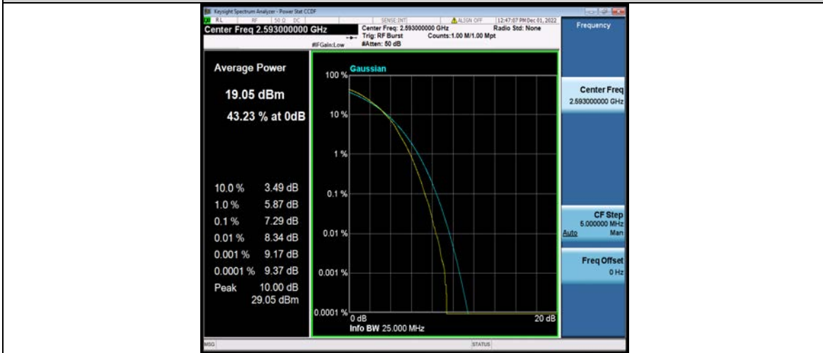
Band41-10MHz-64QAM-41540-1RB#0
