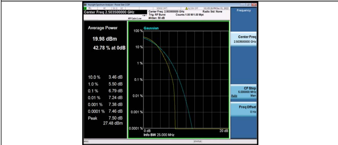
Band41-15MHz-64QAM-39725-75RB#0
