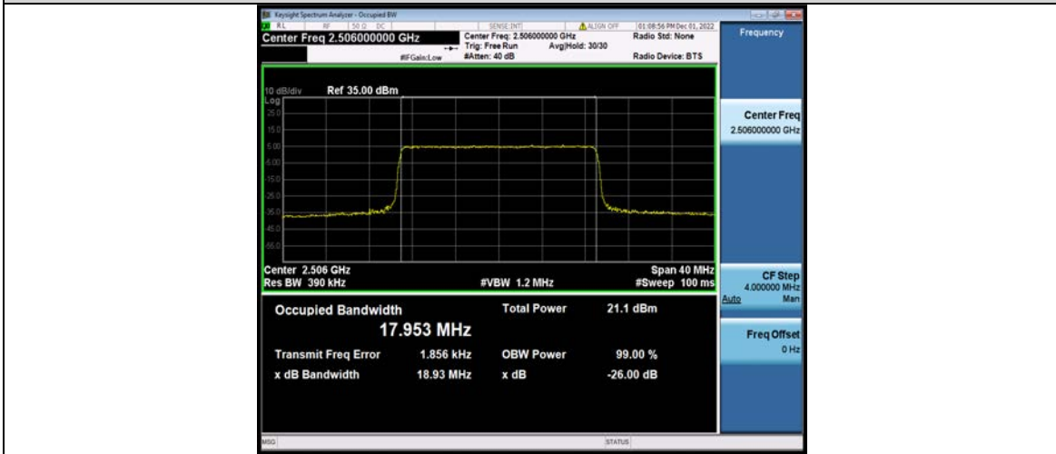
Band41-20MHz-16QAM-40620-100RB#0
