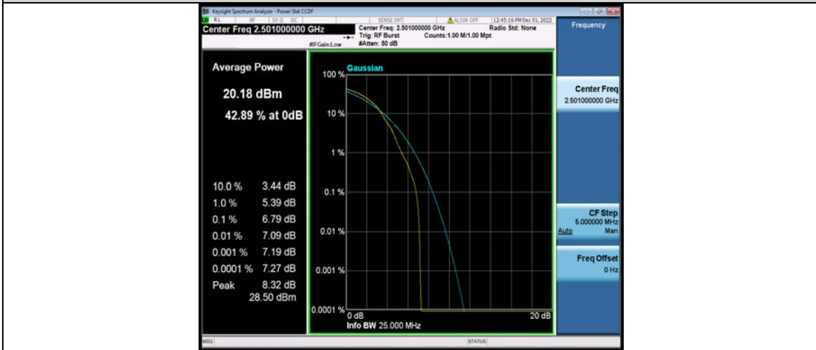
Band41-10MHz-64QAM-39700-50RB#0
