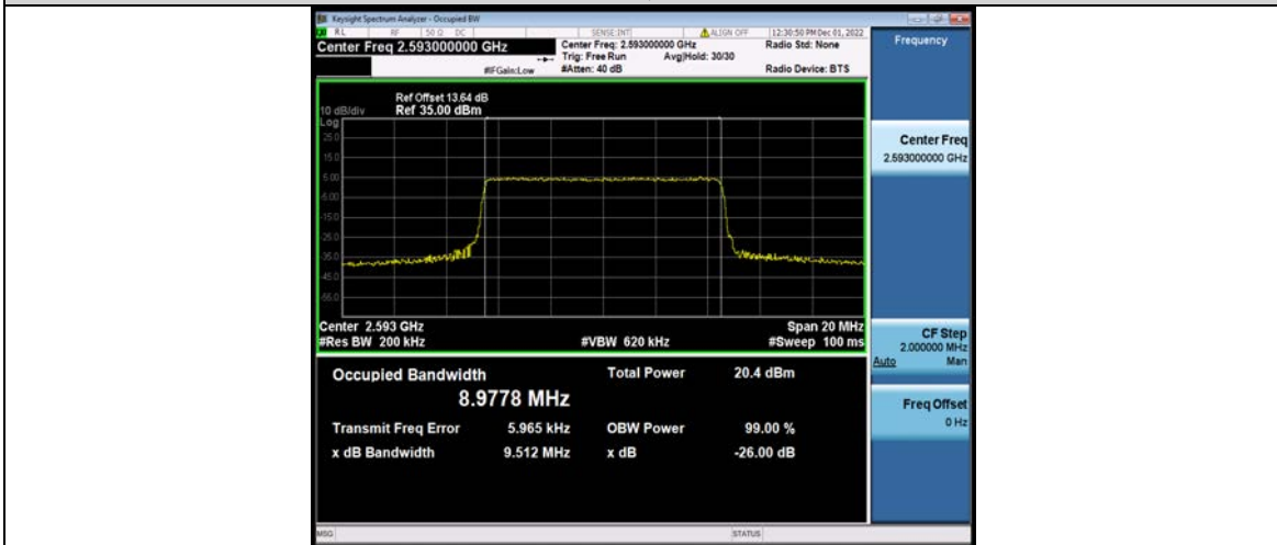
Band41-10MHz-64QAM-41540-50RB#0
