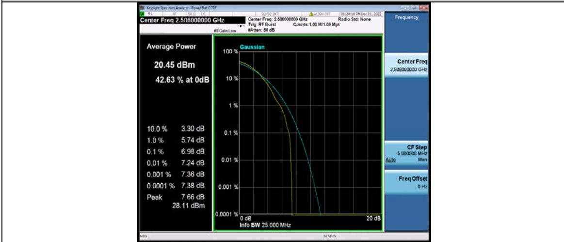
Band41-20MHz-64QAM-39750-100RB#0
