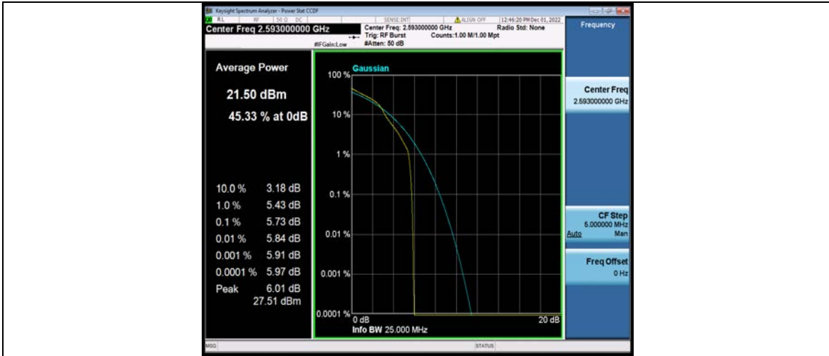
Band41-10MHz-16QAM-40620-50RB#0
