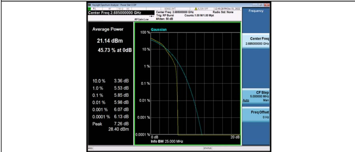
Band41-10MHz-16QAM-41540-50RB#0
