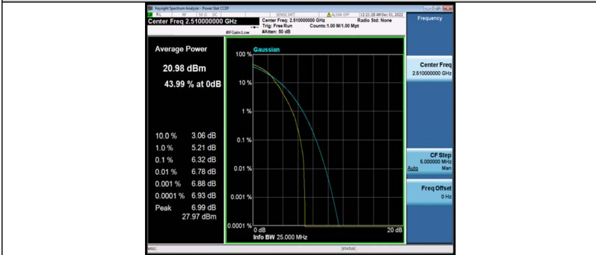
Band7-20MHz-64QAM-20850-100RB#0
