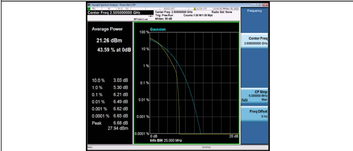
Band7-10MHz-64QAM-20800-50RB#0
