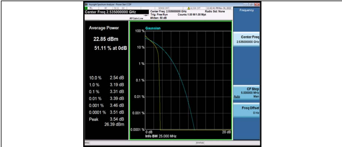
Band7-10MHz-QPSK-21100-50RB#0
