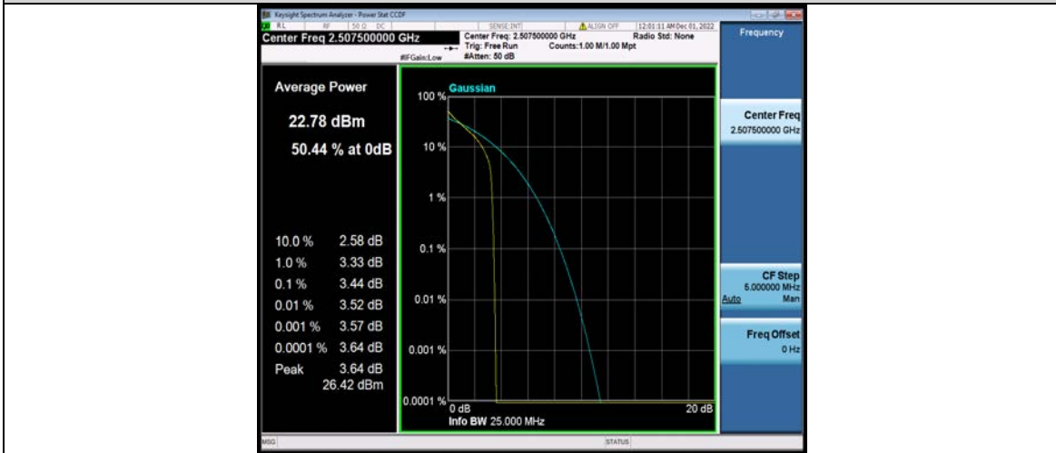
Band7-15MHz-QPSK-20825-75RB#0
