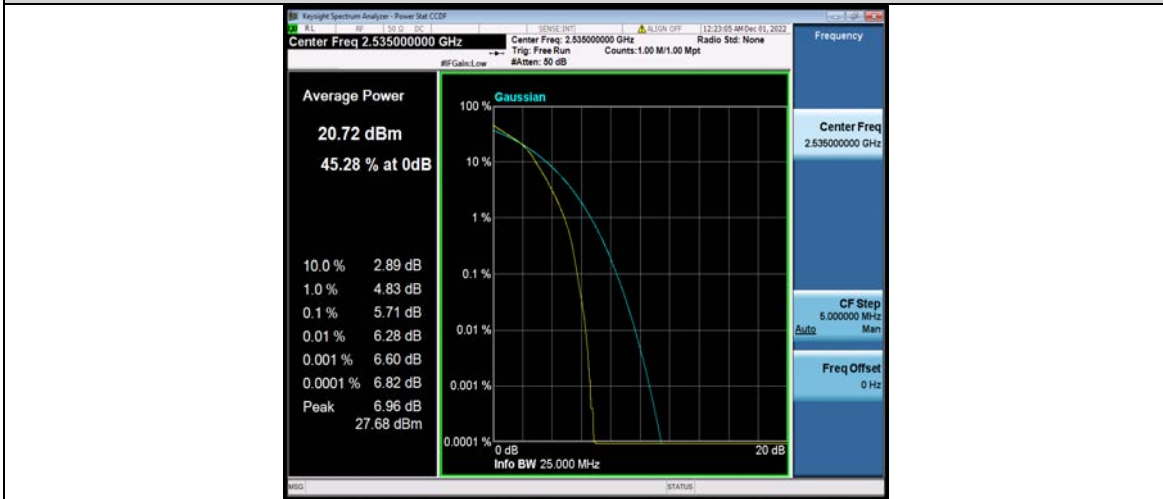
Band7-20MHz-16QAM-21350-1RB#0
