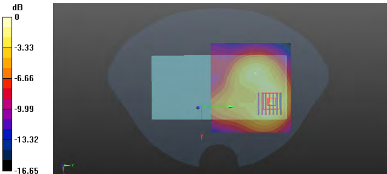
0 dB = 0.350 W/kg
