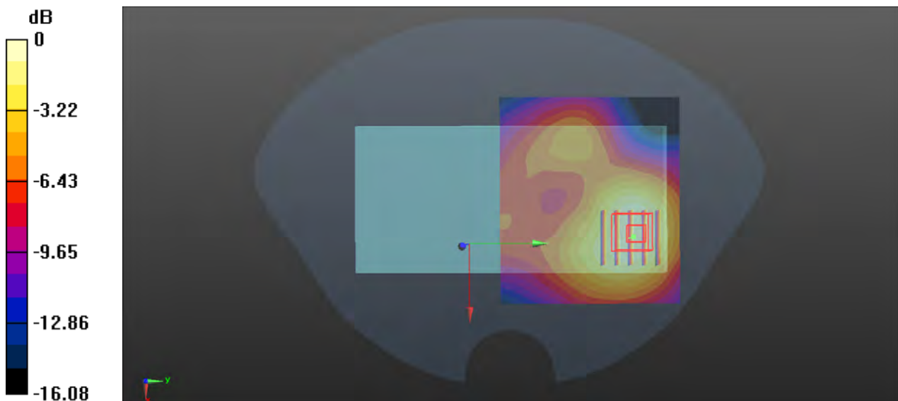
0 dB = 0.129 W/kg
