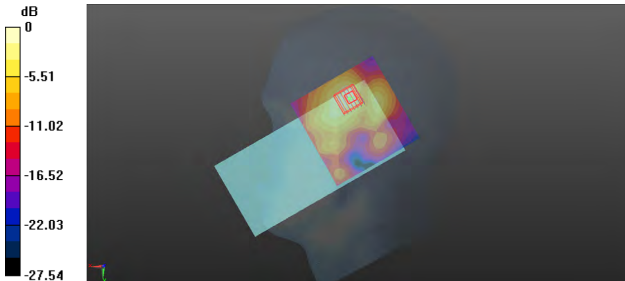
0 dB = 0.839 W/kg
