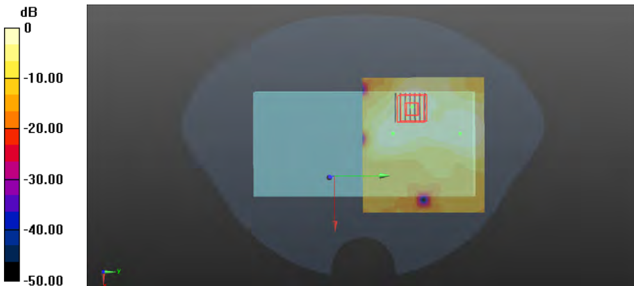
0 dB = 0.202 W/kg
