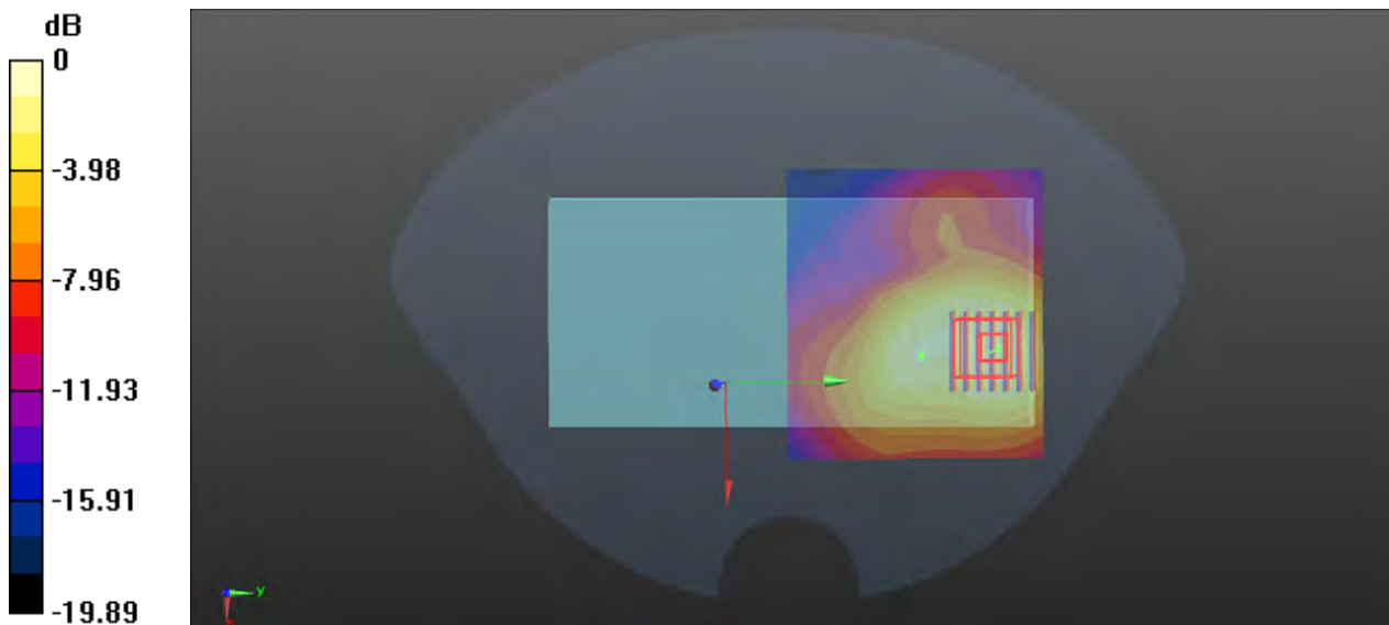
0 dB = 0.309 W/kg
