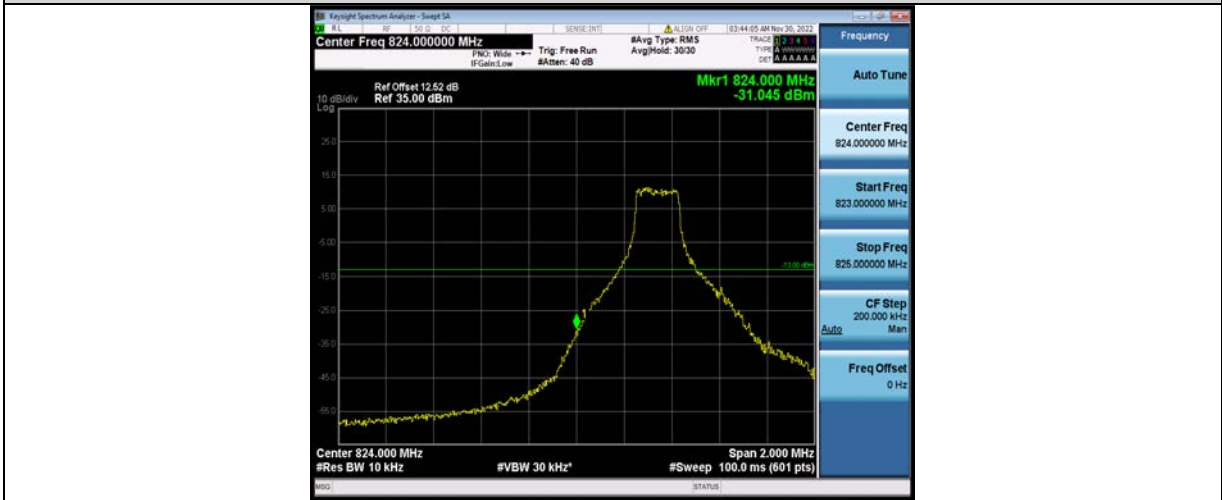
Band26-5MHz-QPSK-26815-25RB#0
