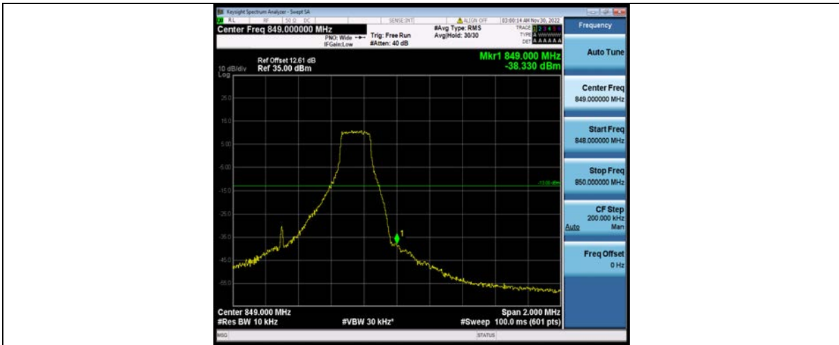
Band26-1.4MHz-QPSK-27033-6RB#0
