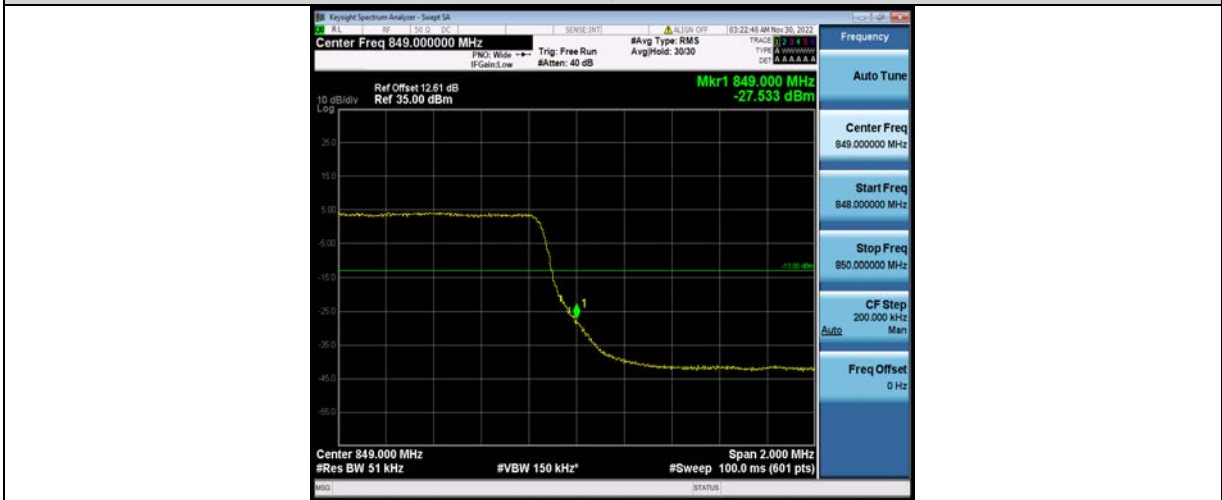
Band26-3MHz-64QAM-26805-1RB#0
