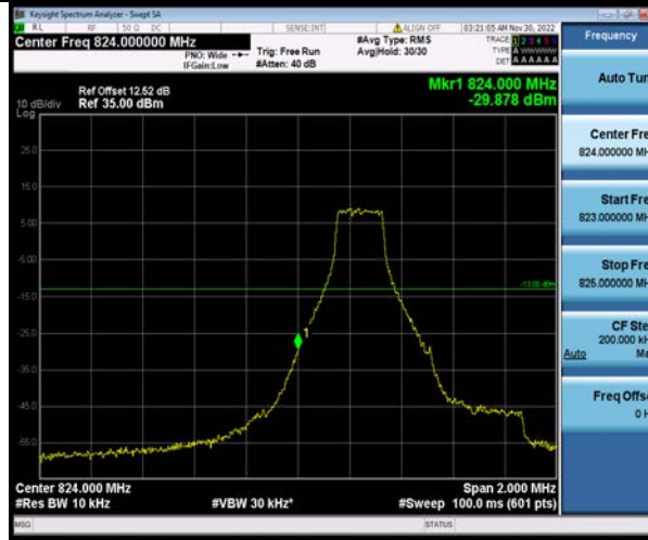
Band26-3MHz-64QAM-26805-15RB#0
