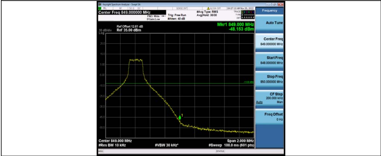
Band26-10MHz-16QAM-26990-50RB#0
