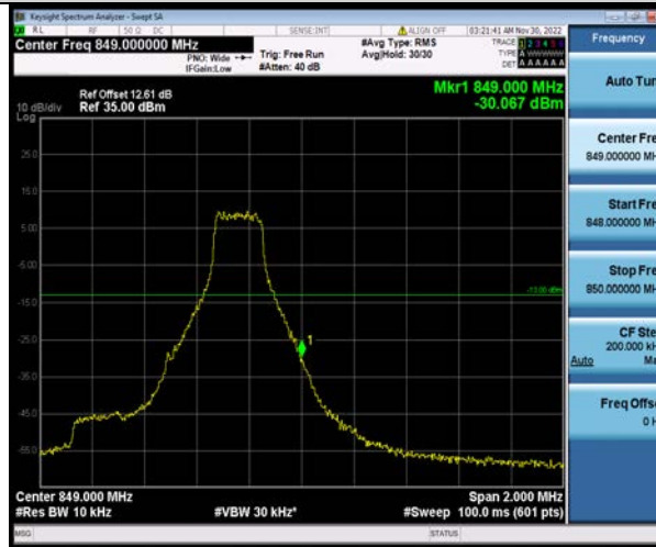
Band26-3MHz-64QAM-27025-15RB#0
