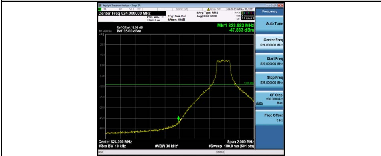
Band26-10MHz-16QAM-26840-50RB#0
