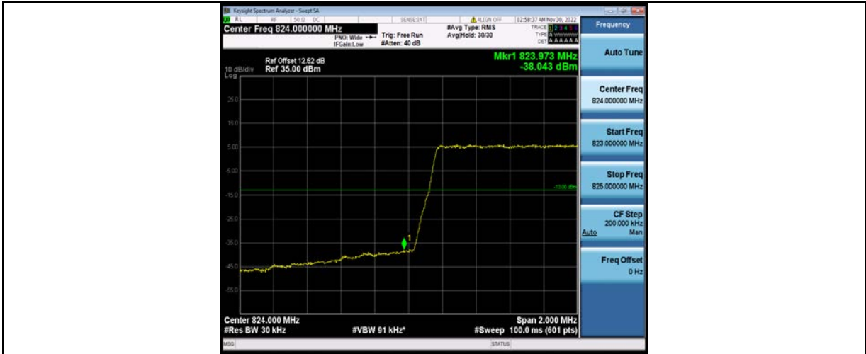
Band26-1.4MHz-16QAM-27033-1RB#5
