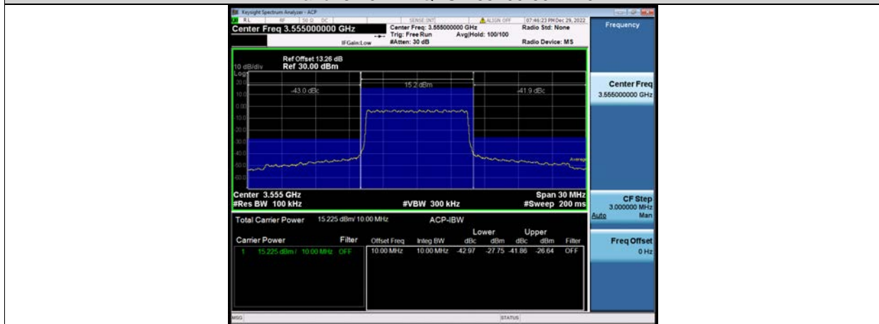
Band48-10MHz-QPSK-55990-1RB#0
