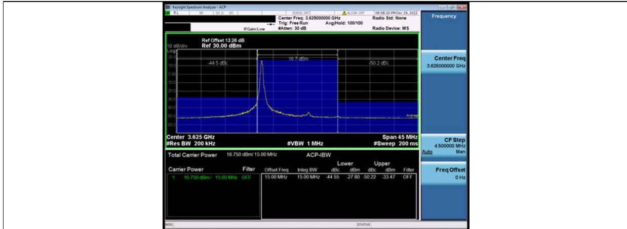
Band48-15MHz-QPSK-55990-75RB#0
