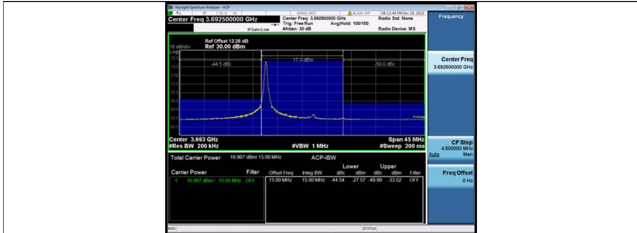
Band48-15MHz-QPSK-56665-75RB#0
