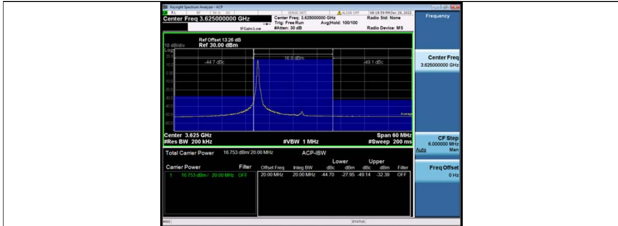
Band48-20MHz-QPSK-55990-1RB#99
