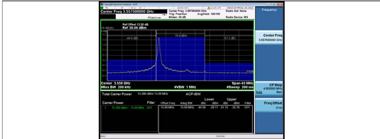
Band48-15MHz-QPSK-55315-75RB#0
