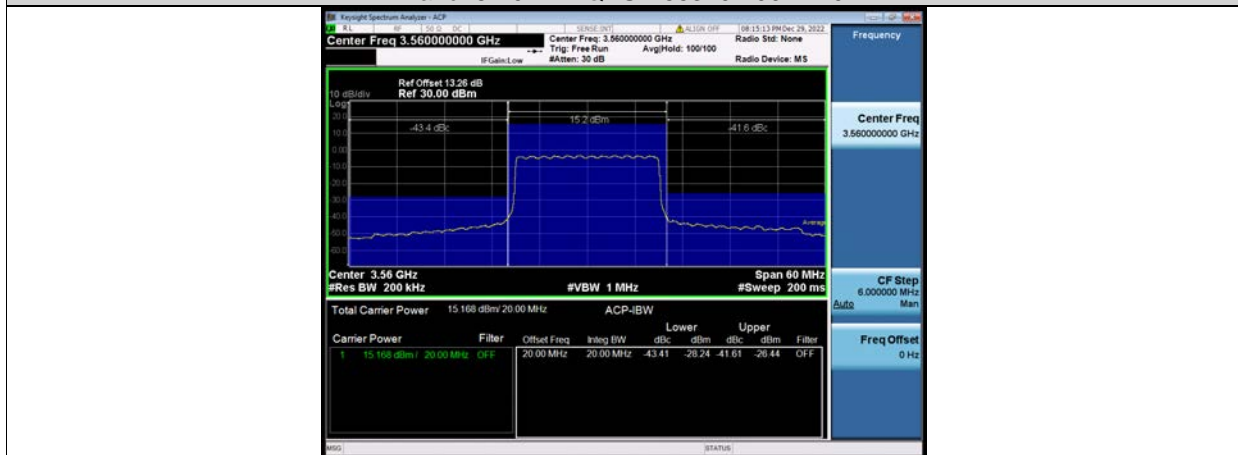
Band48-20MHz-QPSK-55990-1RB#0
