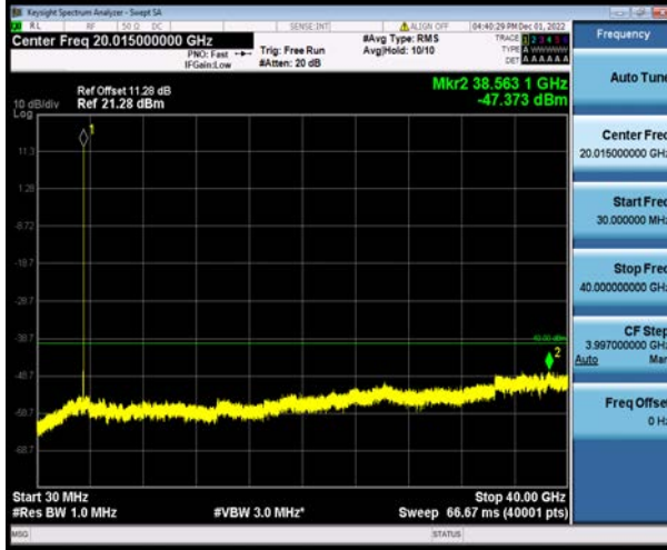
Band48-5MHz-QPSK-55990-1RB#0-Range1:30~40000MHz
