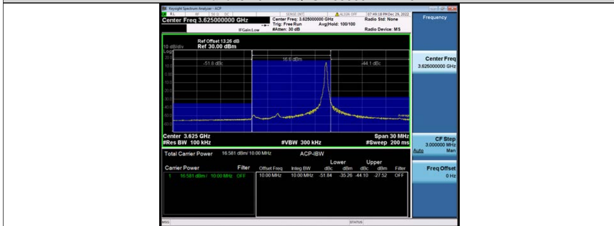
Band48-10MHz-QPSK-55990-50RB#0
