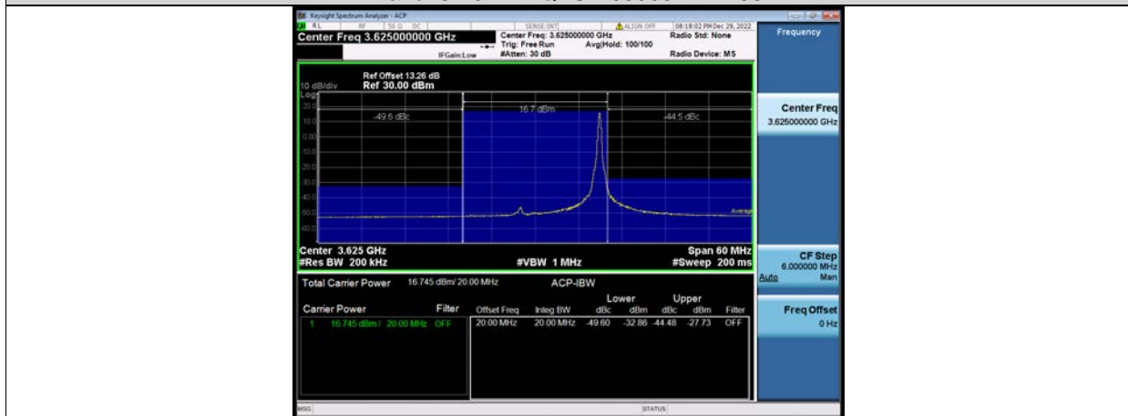
Band48-20MHz-QPSK-55990-100RB#0
