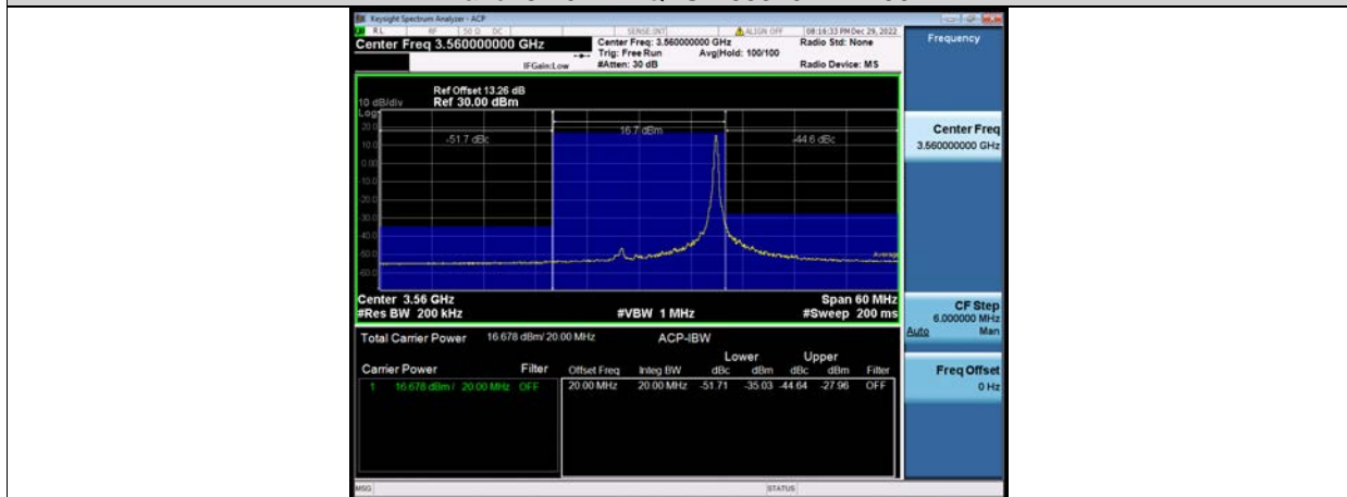
Band48-20MHz-QPSK-55340-100RB#0
