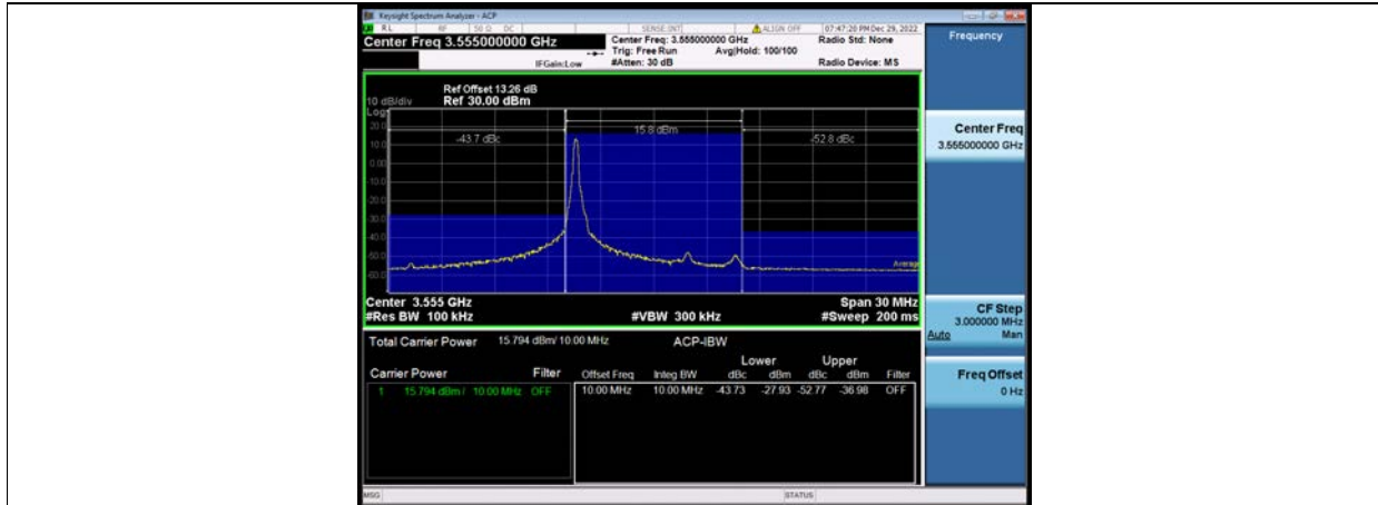
Band48-10MHz-QPSK-55290-1RB#49
