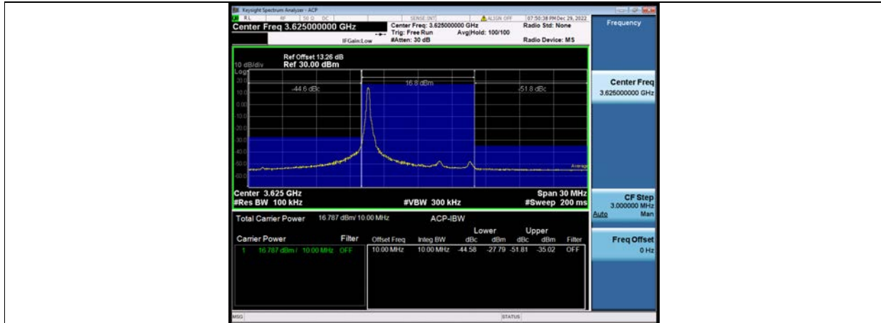
Band48-10MHz-QPSK-55990-1RB#49
