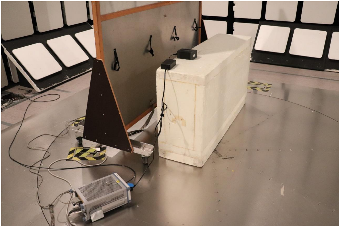
Photograph 5. The EUT and test set-up for conducted emission test
