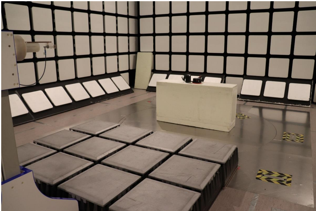
Photograph 9. Radiated Emissions 18 – 26.5 GHz
