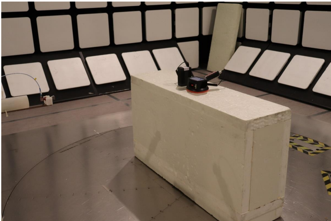
Photograph 10. Radiated Emissions 26.5 – 40 GHz
