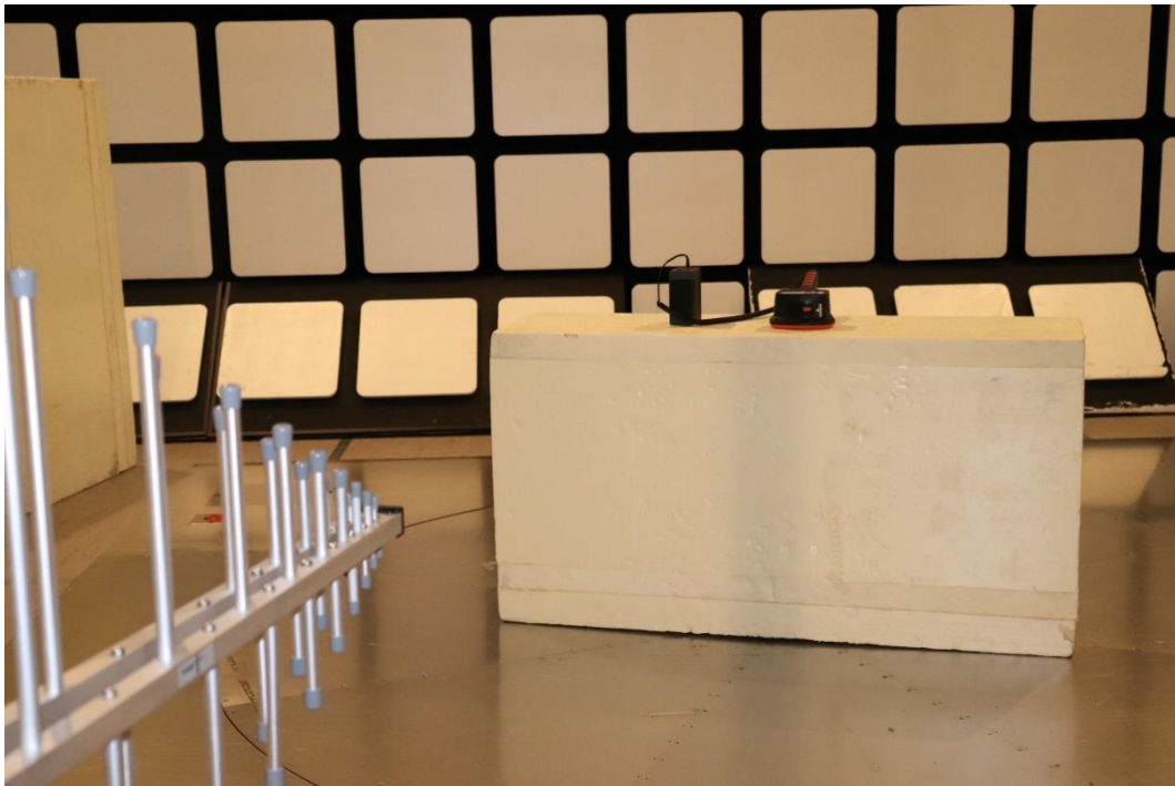
Photograph 7. Radiated Emissions 30 – 1000 MHz
