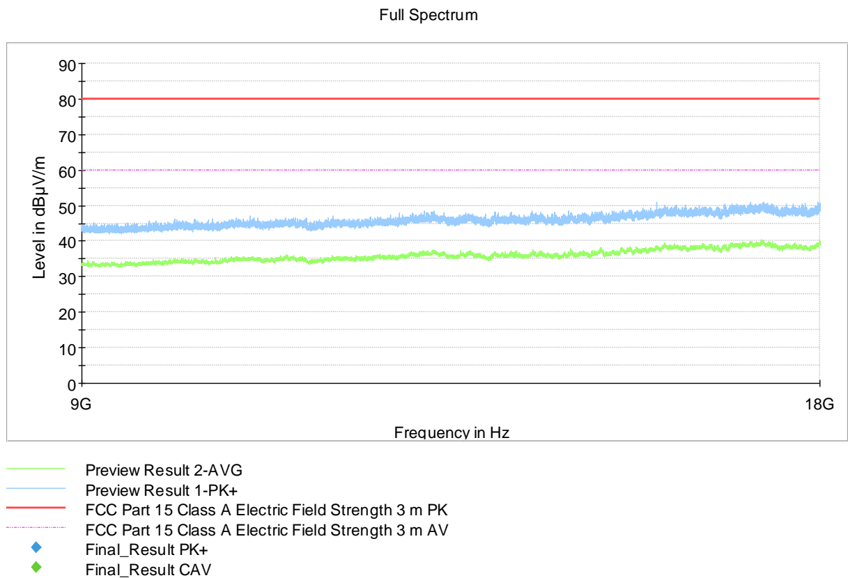
Figure 4: Results with peak and average detectors
