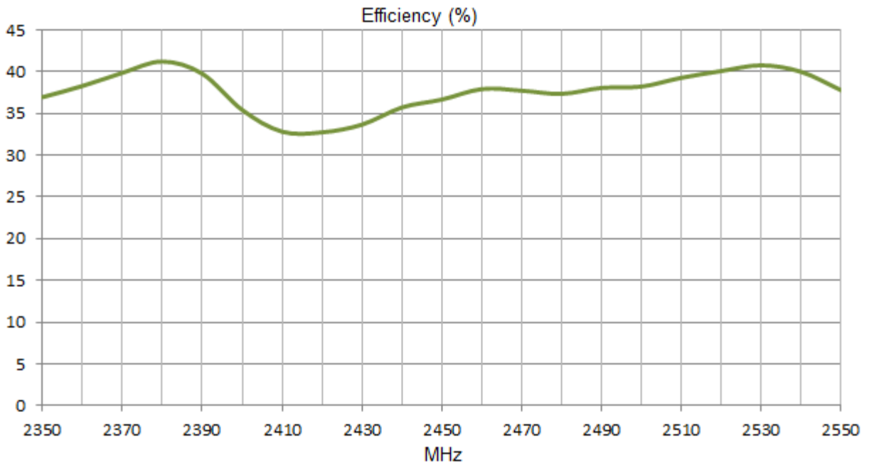
Figure 9. Efficiency of G30 Antenna at 2.4 GHz on metal plate 30x30 cm.
