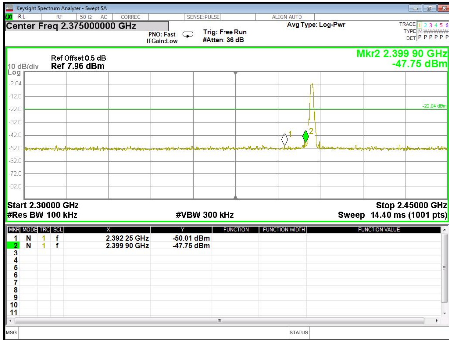
CH01 2402MHZ
