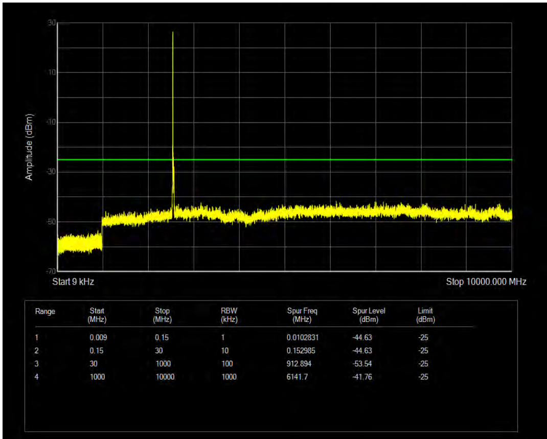
Band41 QAM16 BW=10MHz Channel=40740 RB Size=50 Position=#0
