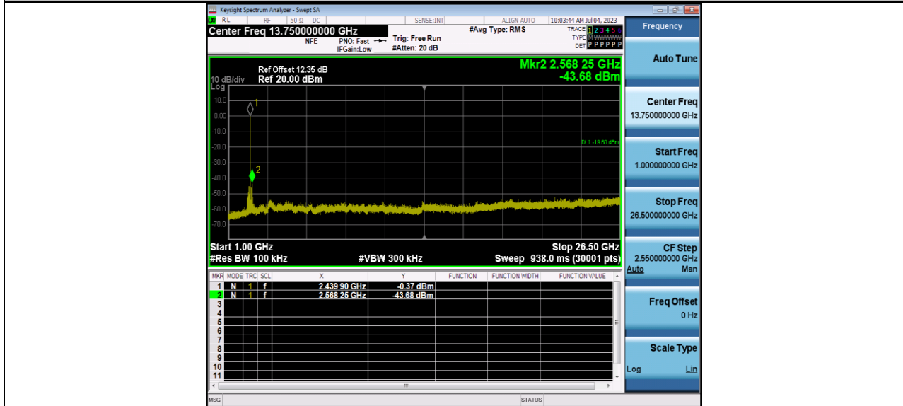
BLE_1M_Ant1_2440_1000~26500
