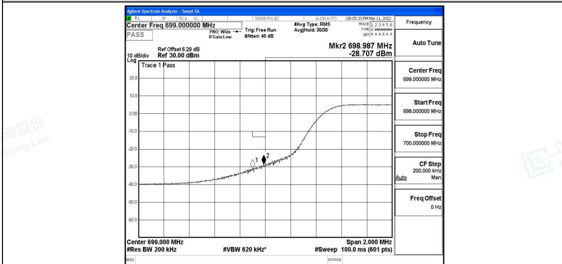
Band12-10MHz-16QAM-23130-50RB#0
