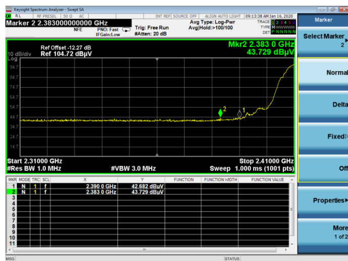
802.11b CHANNEL 1, PEAK
