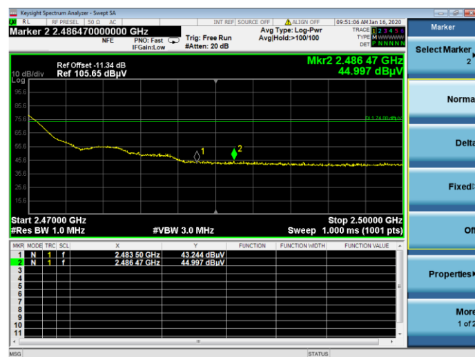
802.11b CHANNEL 11, PEAK
