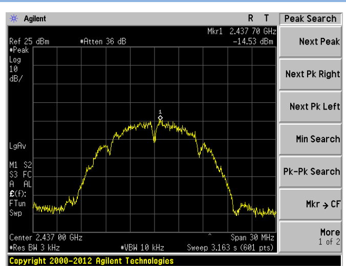
802.11b CHANNEL 6
