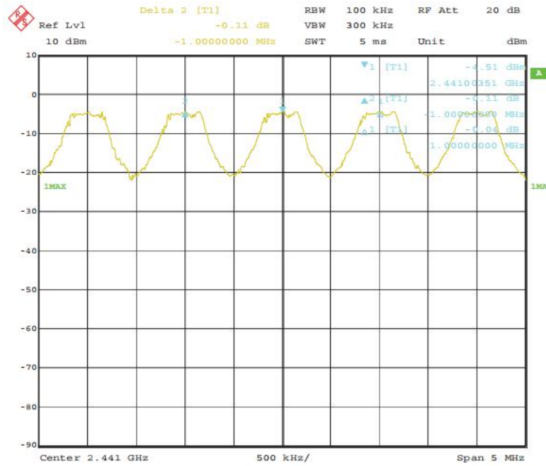
( \pi/4 QPSK) Channel Separation plot
