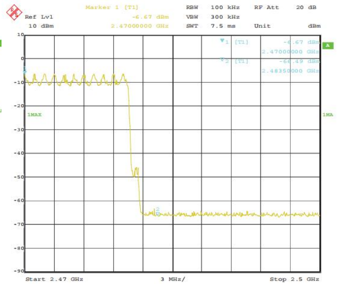
\pi /4-DQPSK: Band Edge-High Channel (Hopping Mode)
