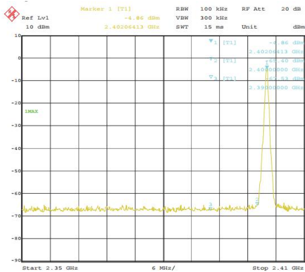
GFSK: Band Edge-Low Channel (Hopping Mode)
