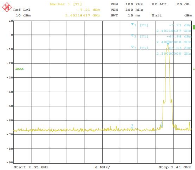
8DQPSK: Band Edge-Low Channel
