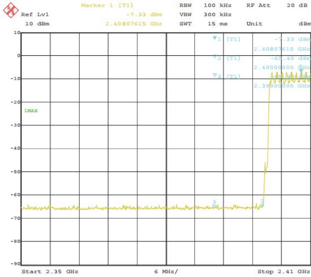
\pi /4-DQPSK: Band Edge-Low Channel (Hopping Mode)
