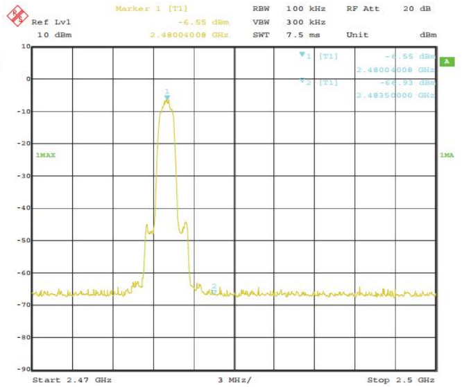
8DQPSK: Band Edge-High Channel
