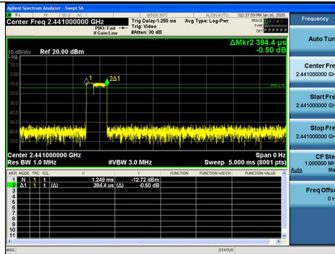
2-DH1
