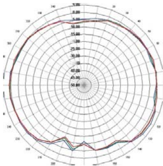
XZ-Plane Gain.
