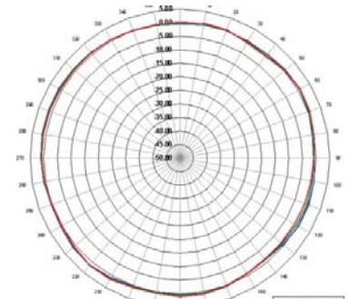
XY-Plane Gain
